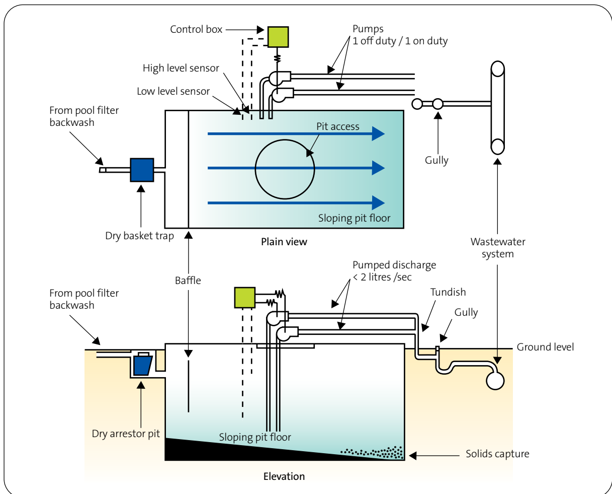
Figure 21 – Key features of a typical backwash water holding tank
