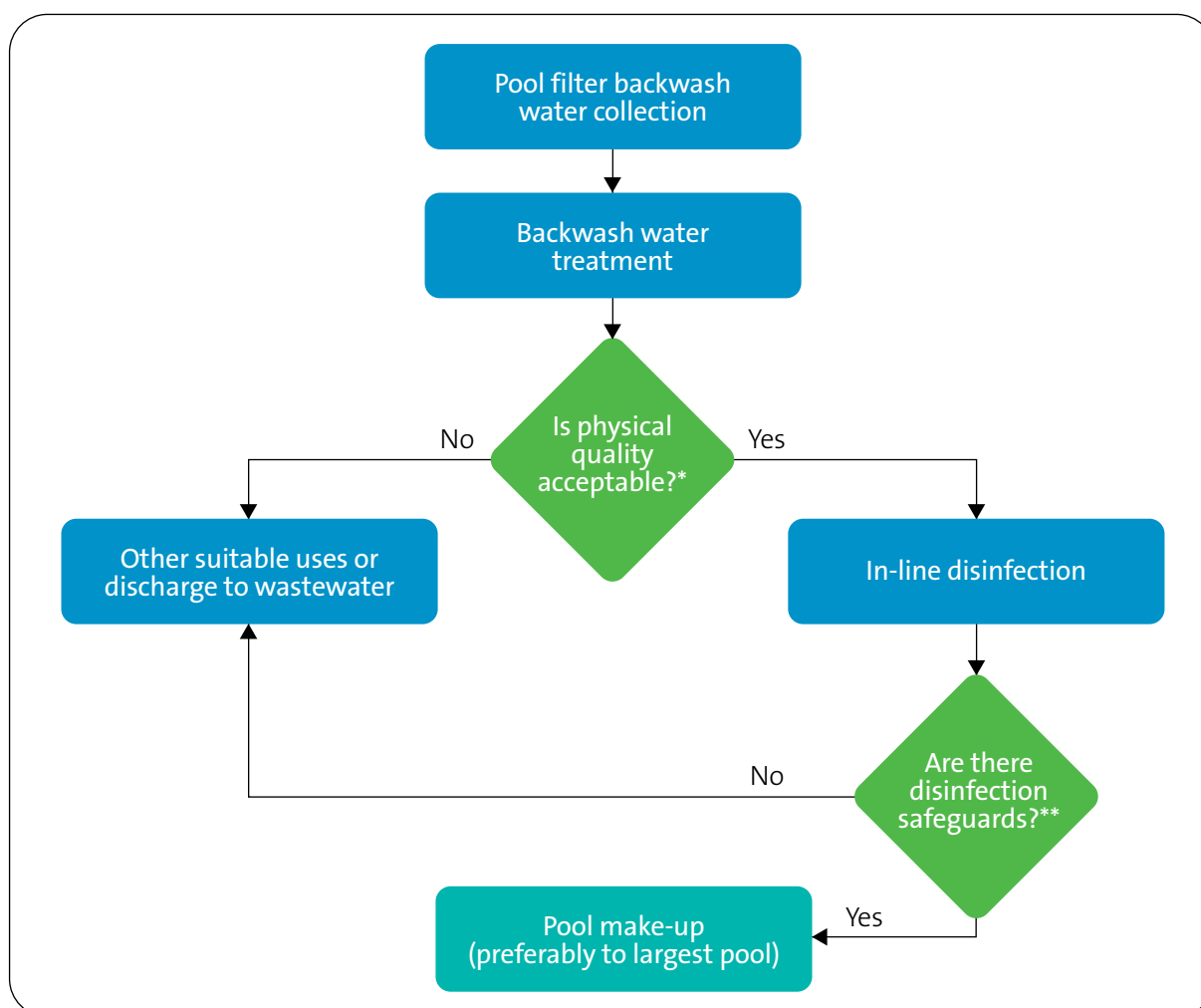
Figure 29 – Deciding how to use treated backwash water
