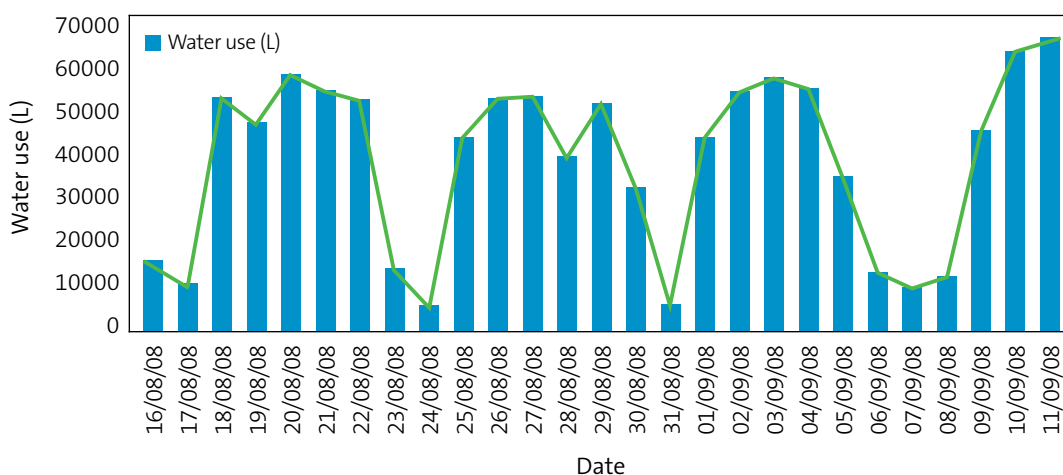
Figure 8 – A typical graph of water use information from a data logger
