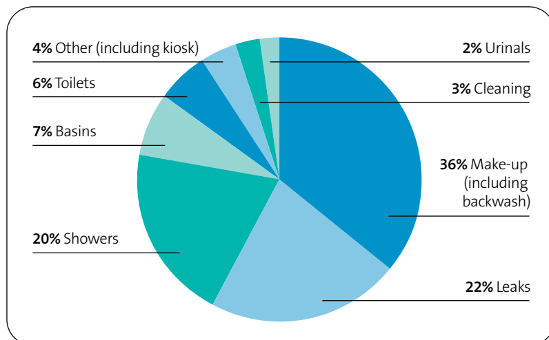
Figure 2 – Water use breakdown of a typical aquatic centre
