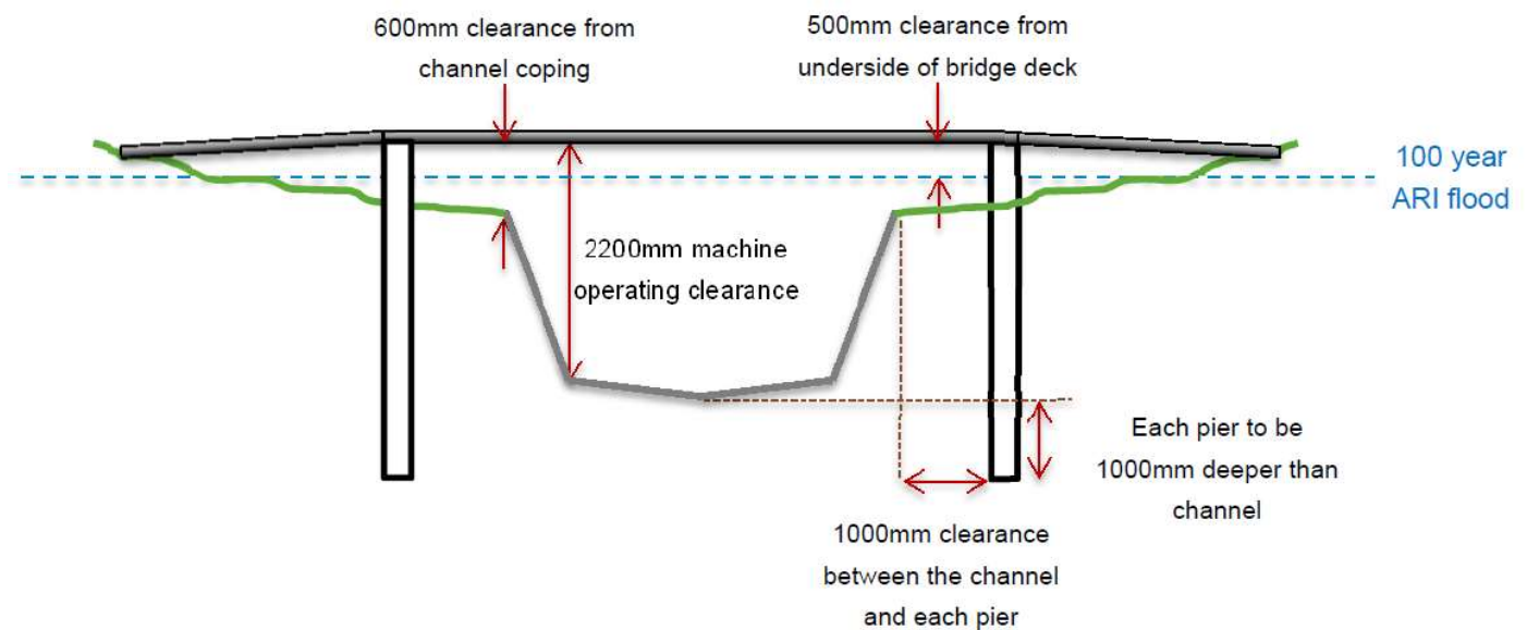
Figure 1 – Minimum clearances
