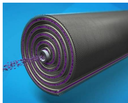
Spiral wound layers in a RO membrane module. The flow of water molecules is shown in purple.
