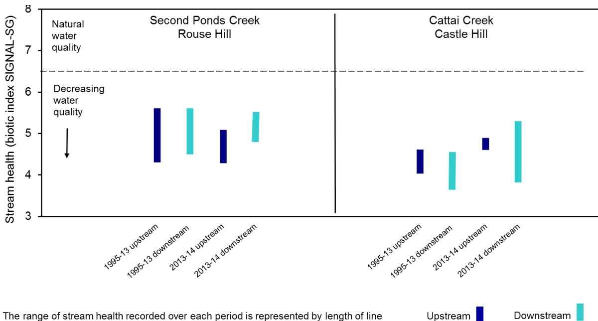
Figure 1-23 Stream health in the Cattai Creek catchment
