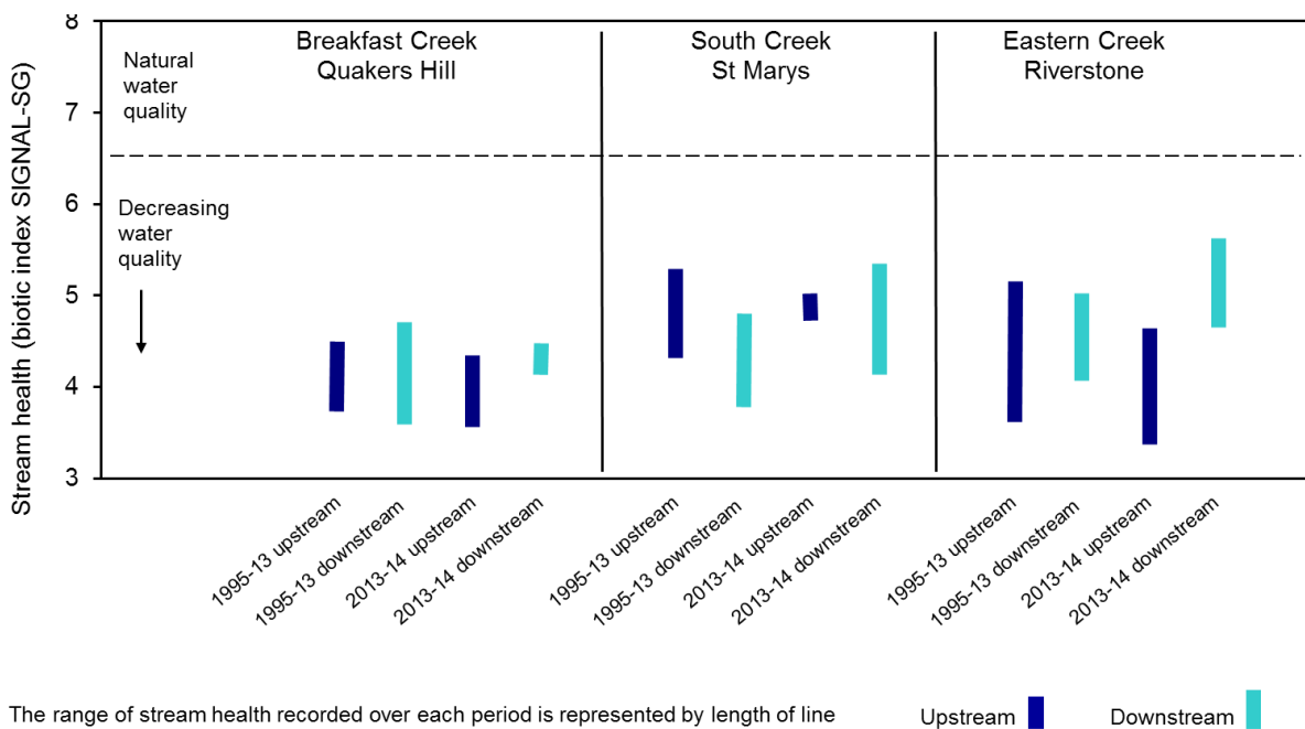
Figure 1-22 Stream health in the South Creek catchment
