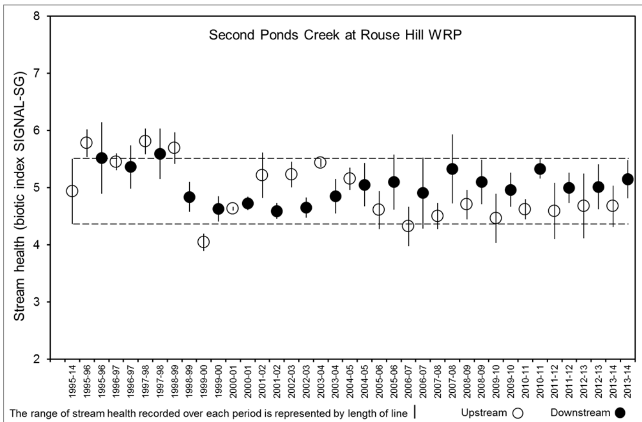
Figure 4-8 Ecological monitoring control chart for Second Ponds Creek at Rouse Hill
