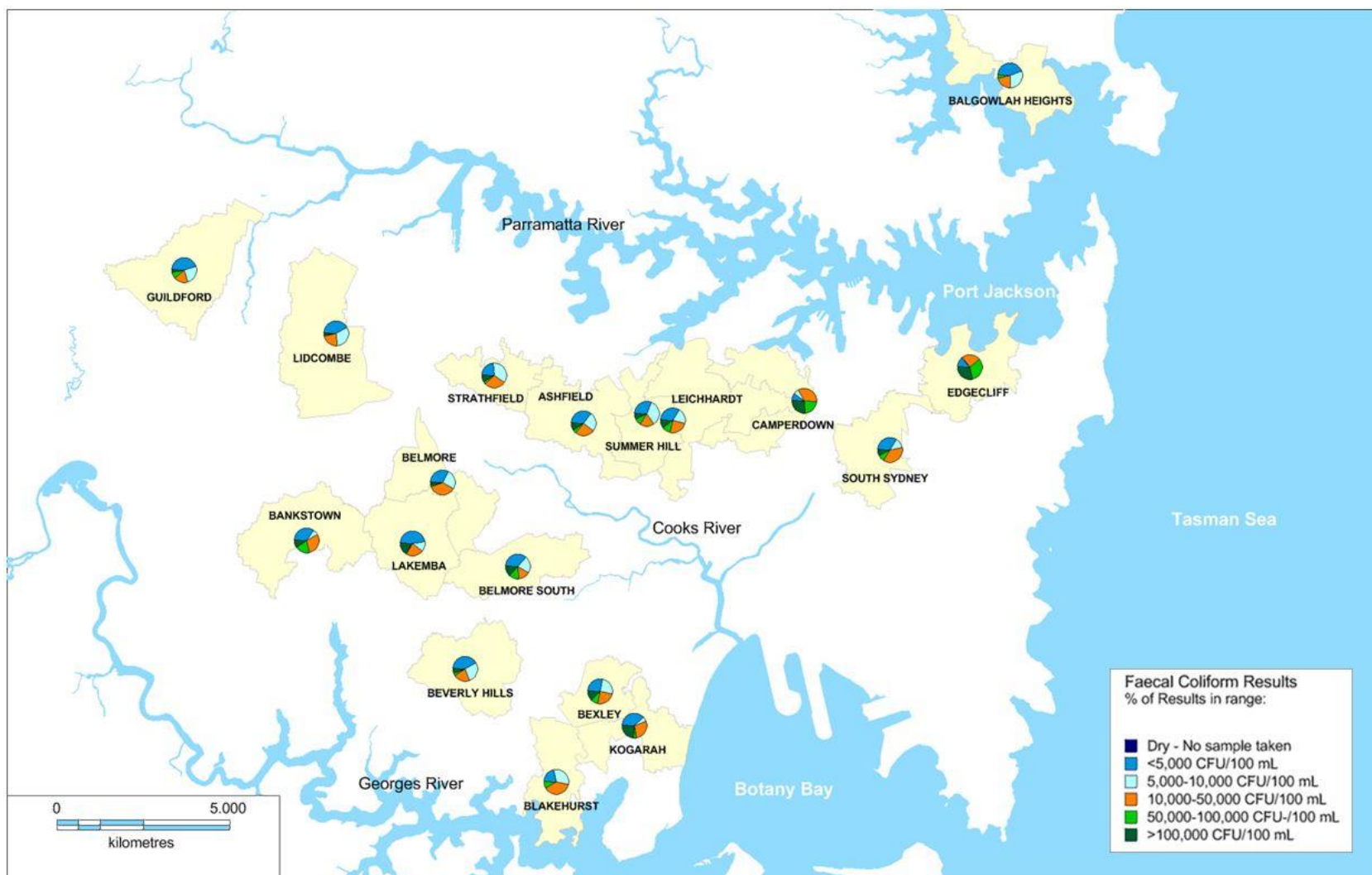
Figure 1-34 Central and southern Sydney SCAMPS that have exceeded the faecal coliform threshold of 5000 cfu/100 mL more than 50% of the time since 2006, with proportion of results exceeding shown
