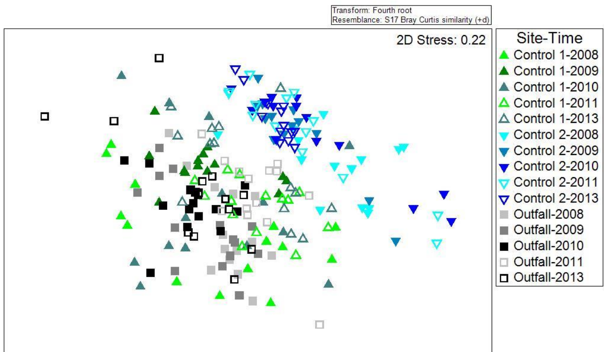
Figure 2-4 Two-dimensional ordination plot of rocky intertidal community structure at Shellharbour outfall and two control sites for years 2008 to 2011 and 2013, with site and year colour coded
