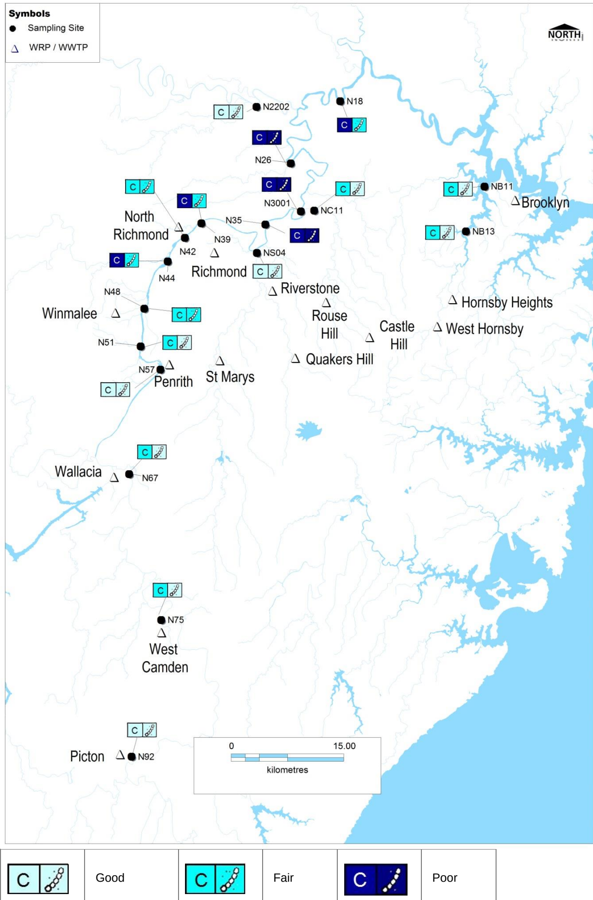
Figure 1-27 Water quality ratings based on chlorophyll a and cyanobacteria at Hawkesbury Nepean River monitoring sites (2013-14)
