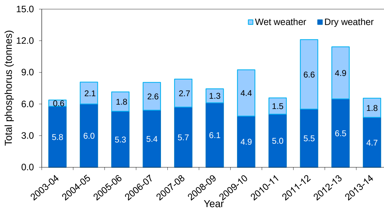
Figure 1-7 Previous ten years of total phosphorus loads from all inland plants
