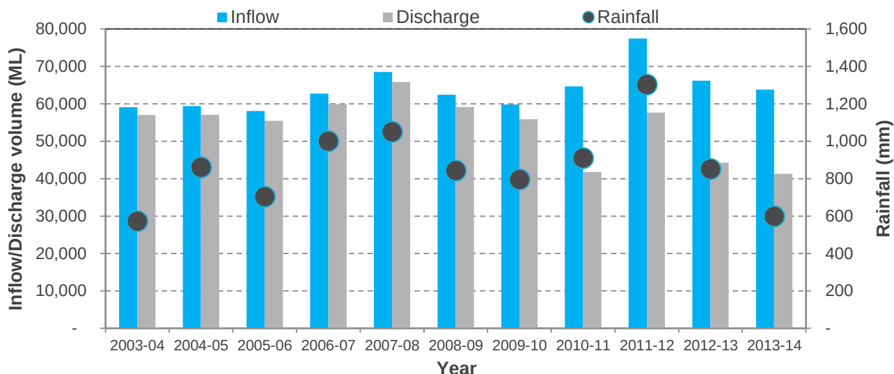
Figure 1-5 Previous ten years of wastewater inflow and discharge volumes from all inland plants and rainfall in the inland catchments
