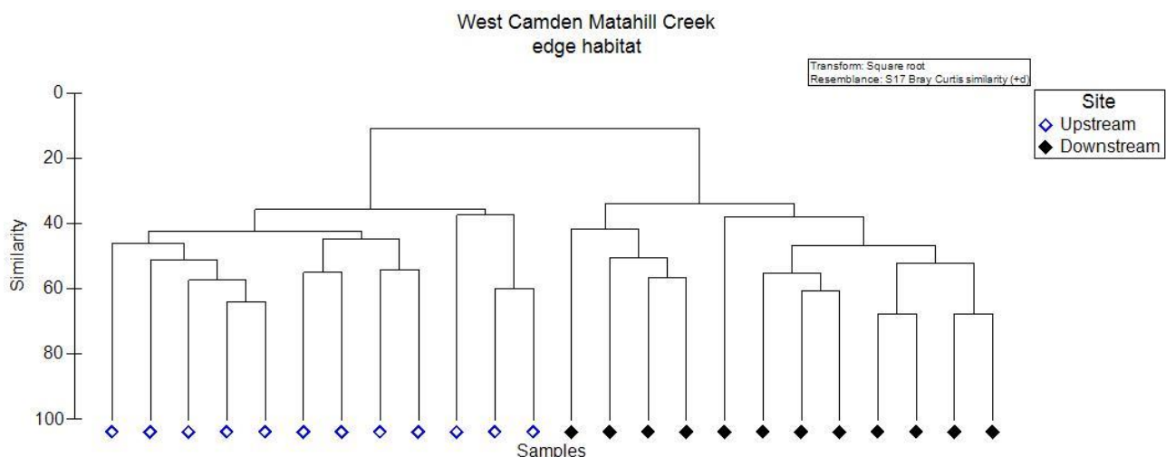
Figure 4-20 Tree diagram of freshwater macroinvertebrate community structure of Matahill Creek upstream and downstream sites of West Camden plant
