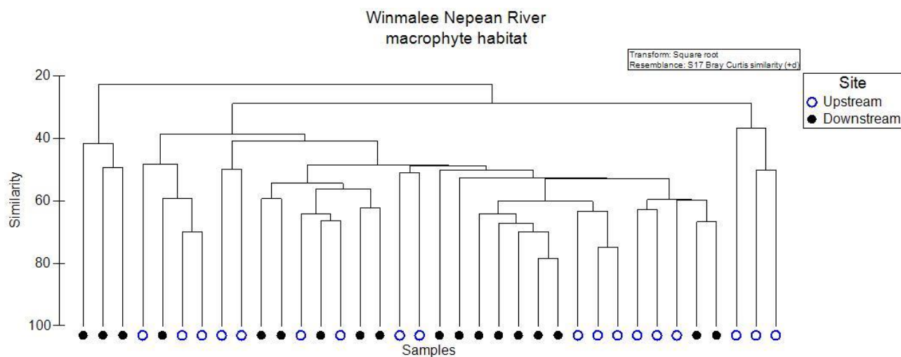
Figure 4-24 Tree diagram of freshwater macroinvertebrate macrophyte habitat community structure of Nepean River upstream and downstream sites of Winmalee plant
