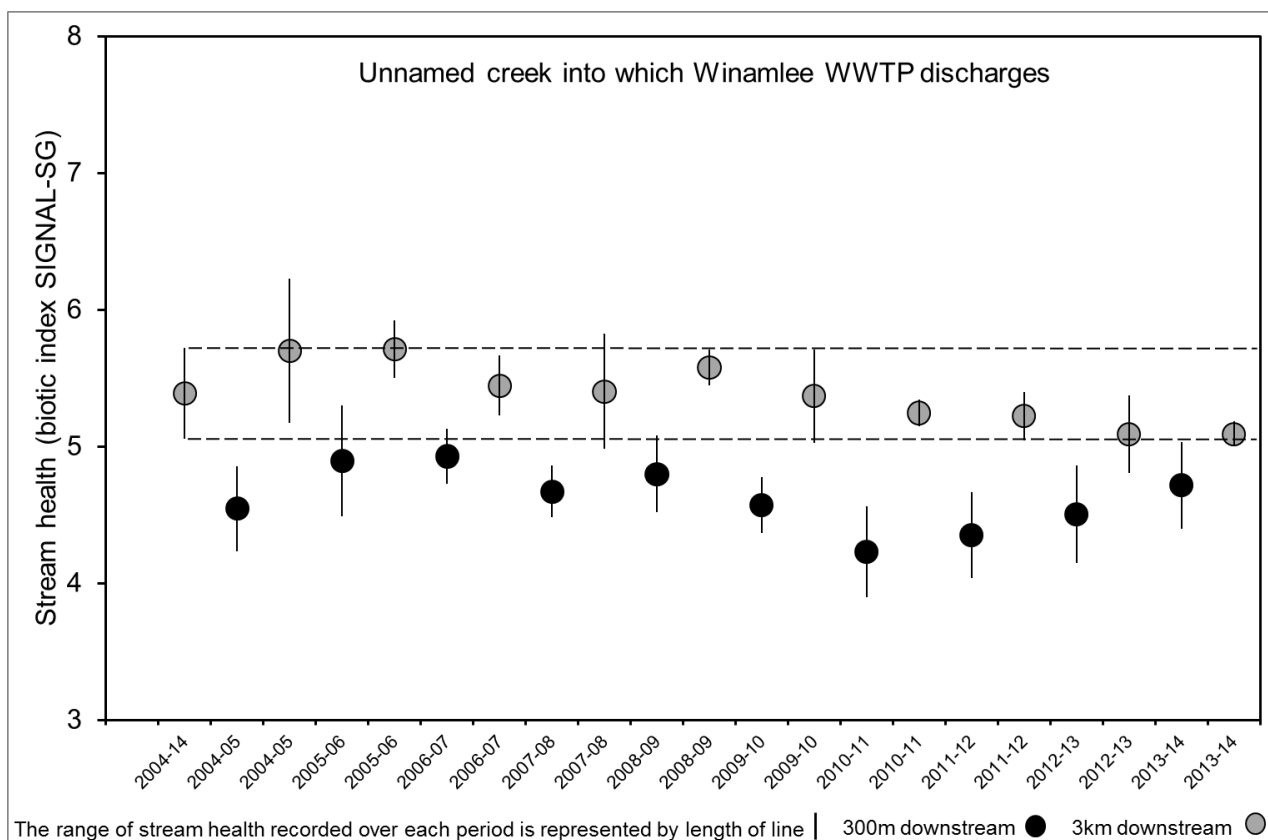
Figure 4-4 Ecological monitoring control chart for unnamed creek at Winmalee
