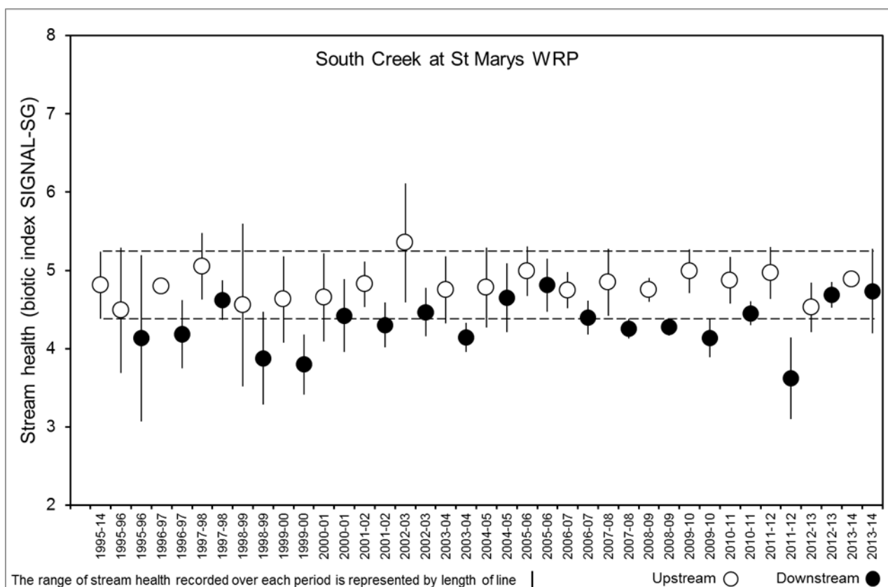
Figure 4-11 Ecological monitoring control chart for South Creek at St Marys
