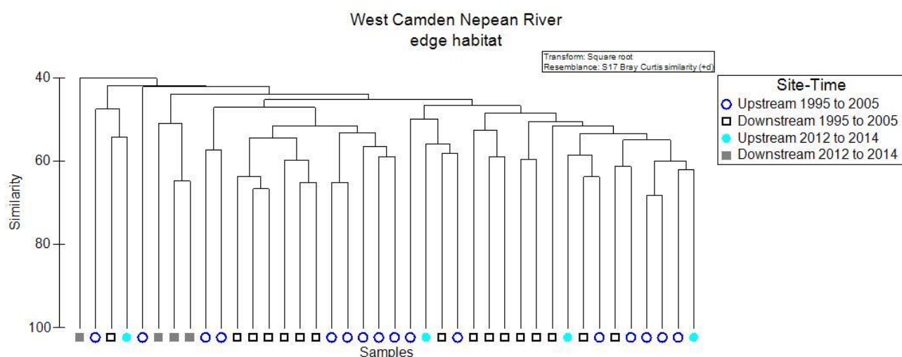
Figure 4-18 Tree diagram from classification analysis of freshwater macroinvertebrate community structure of Hawkesbury Nepean River upstream and downstream sites of West Camden plant for two periods (Period 1 data 1995 to 2005 and Period 2 data from 2012 to 2014)
