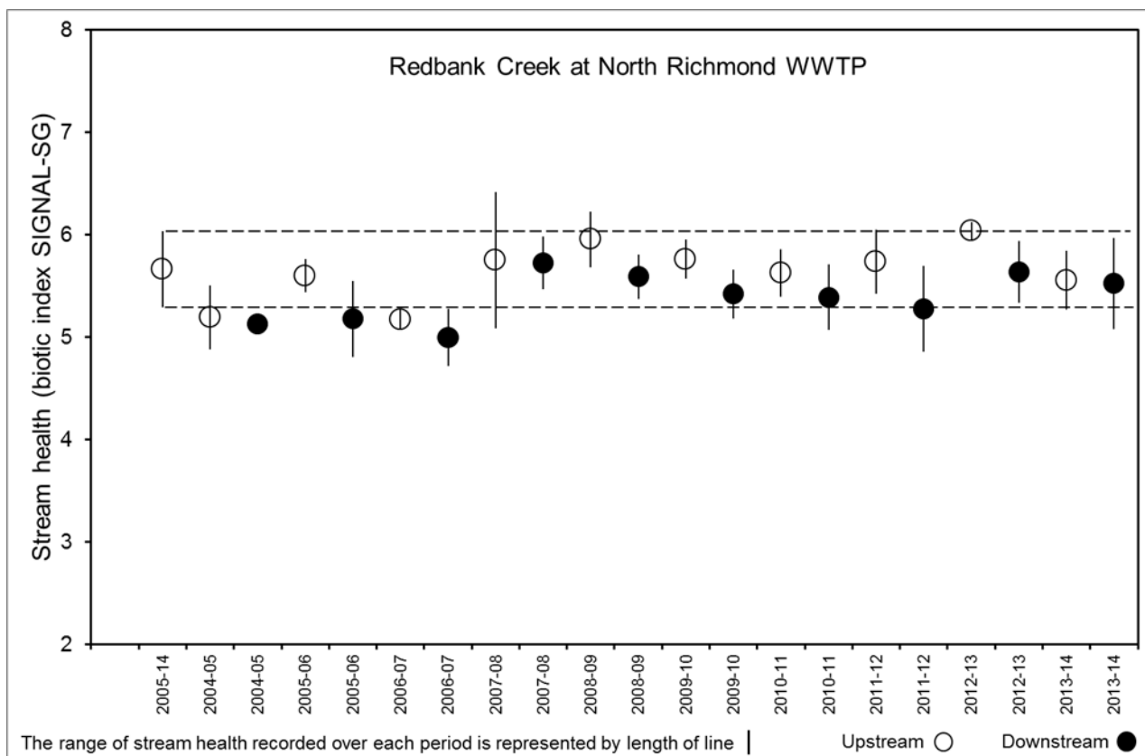
Figure 4-15 Ecological monitoring control chart for Redbank Creek at North Richmond
