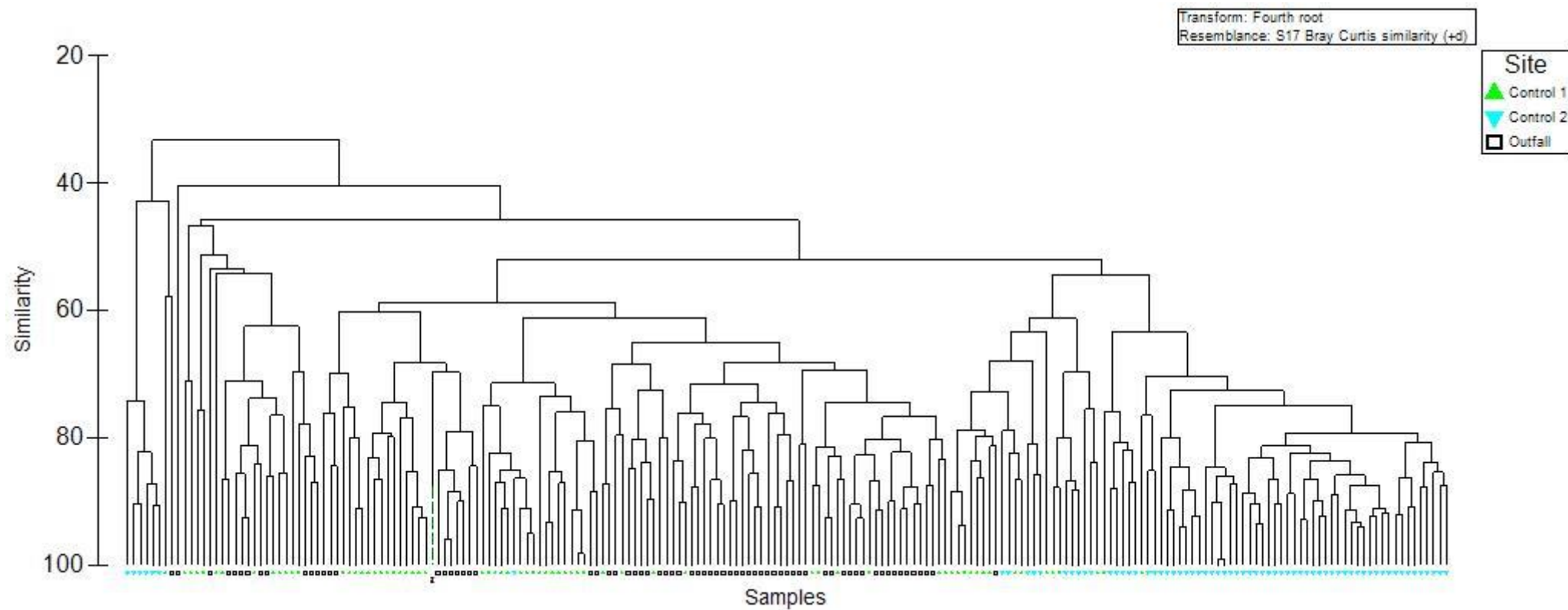
Figure 2-6 Tree diagram of rocky intertidal community structure at Shellharbour outfall and two control sites for years 2008 to 2011 and 2013, with site colour coded
