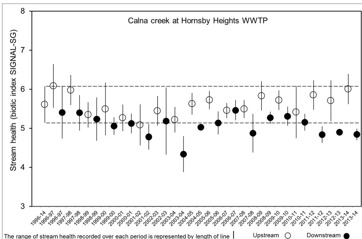
Figure 4-5 Ecological monitoring control chart for Calna Creek at Hornsby Heights
