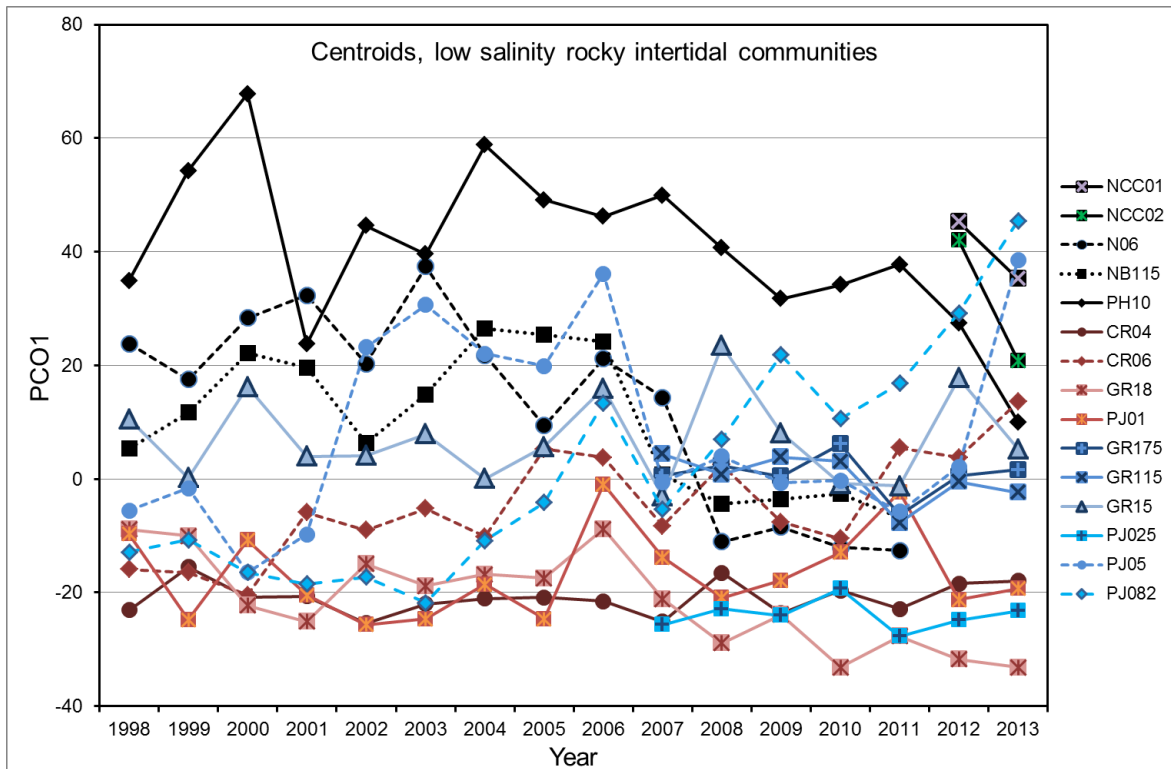
Figure 3-1 Year plotted against Principal Coordinates Analysis axis 1 of distance among centroids for sites of the relatively lower salinity zone
