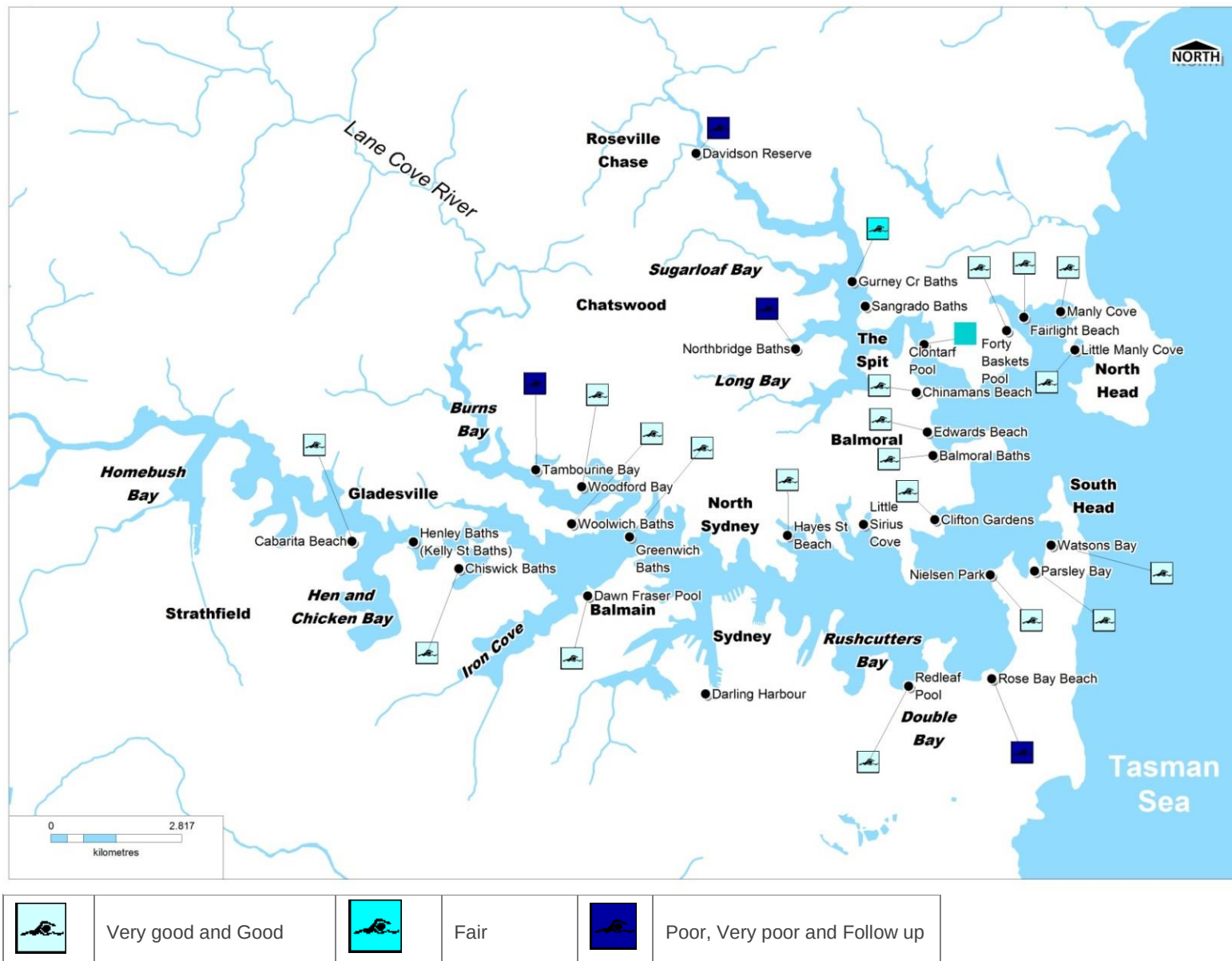
Figure 1-14 Beach Suitability Grades for Sydney Harbour
