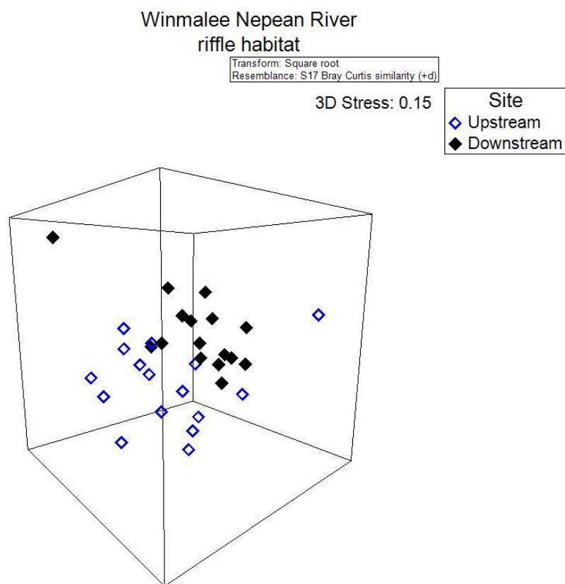
Figure 4-23 Three-dimensional ordination plot of freshwater macroinvertebrate riffle habitat community structure of Hawkesbury Nepean River upstream and downstream sites of Winmalee plant
