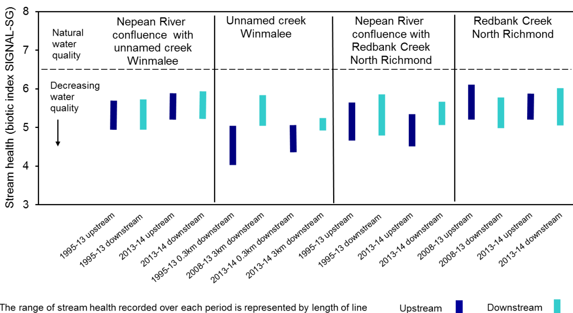
Figure 1-20 Stream health in the lower Hawkesbury Nepean River catchment
