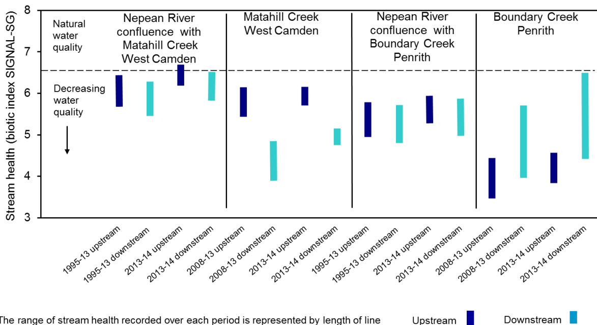
Figure 1-19 Stream health in the upper Hawkesbury Nepean River catchment
