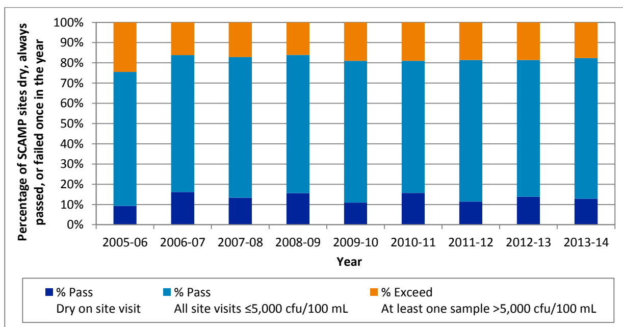
Figure 1-32 Percentage of SCAMPs that were dry, returned faecal coliform results below the 5,000 cfu/100 mL threshold, or exceeded the threshold over the history of the program
