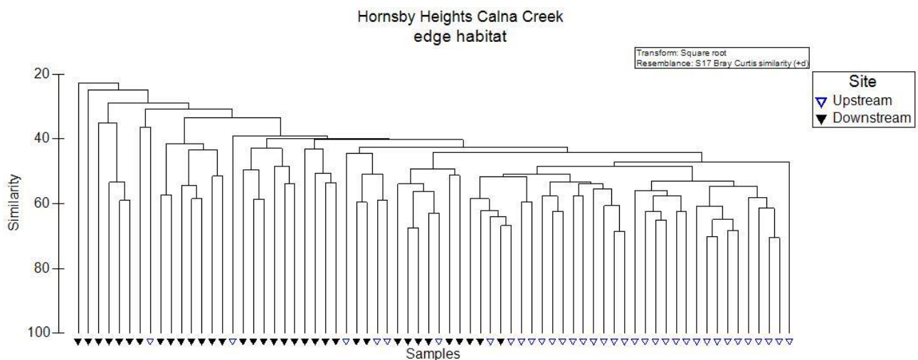
Figure 4-33 Tree diagram of freshwater macroinvertebrate edge habitat community structure of Calna Creek upstream and downstream sites of Hornsby Heights plant
