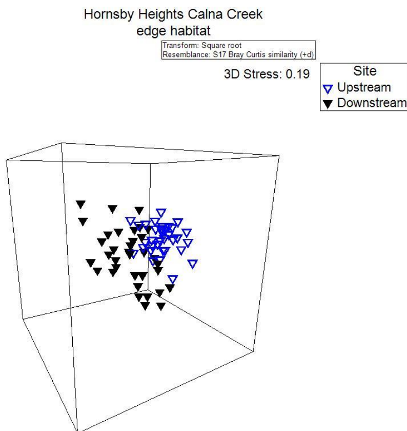
Figure 4-31 Three-dimensional ordination plot of freshwater macroinvertebrate edge habitat community structure of Calna Creek upstream and downstream sites of Hornsby Heights plant
