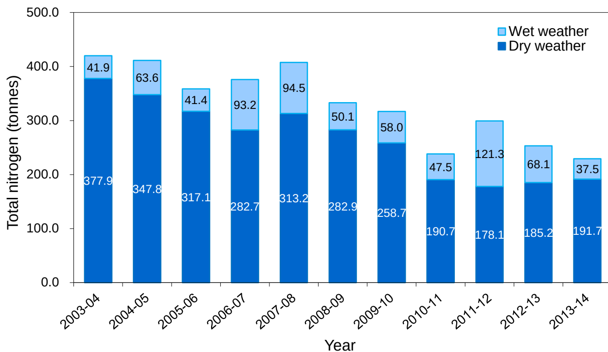
Figure 1-6 Previous ten years of total nitrogen loads from all inland plants
