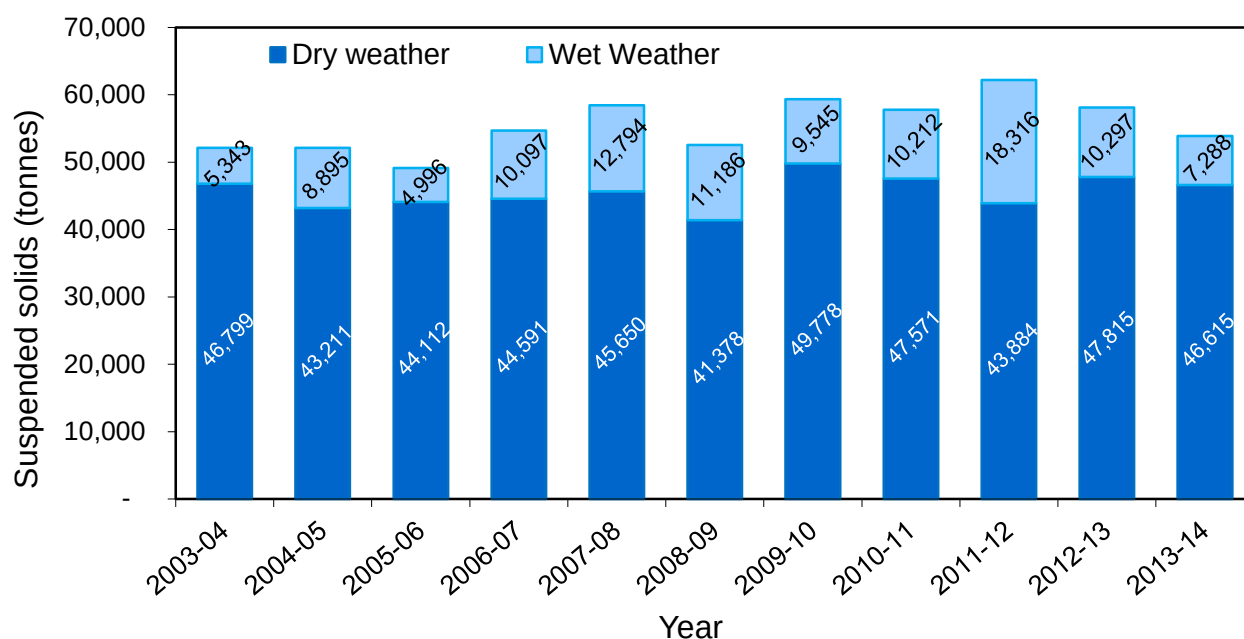
Figure 1-4 Previous ten years of total suspended solids loads from all ocean plants
