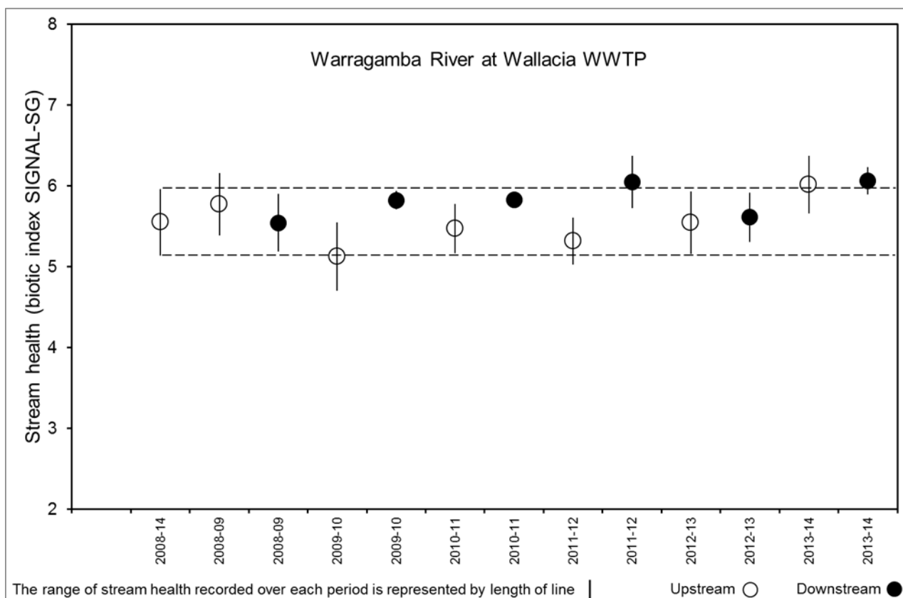
Figure 4-12 Ecological monitoring control chart for Warragamba River at Wallacia
