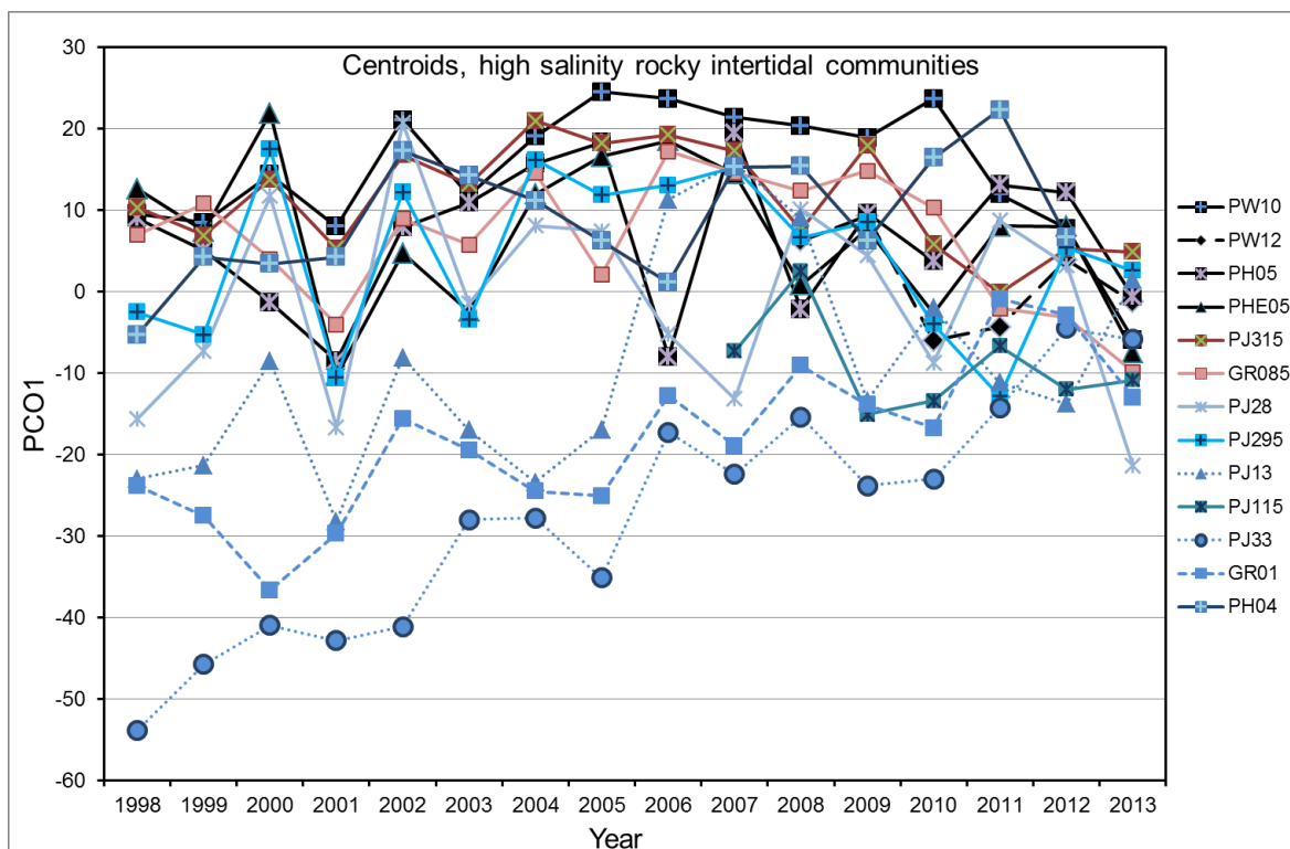
Figure 3-2 Year plotted against Principal Coordinates Analysis axis 1 of distance among centroids for sites of the relatively higher salinity zone
