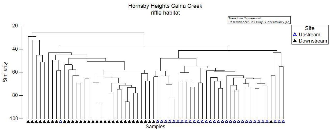
Figure 4-34 Tree diagram of freshwater macroinvertebrate riffle habitat community structure of Calna Creek upstream and downstream sites of Hornsby Heights plant
