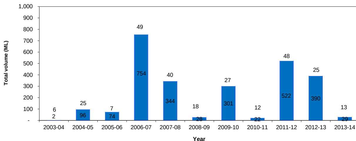
Figure 1-31 Previous ten years of modelled wet weather overflow volumes by all inland wastewater systems
