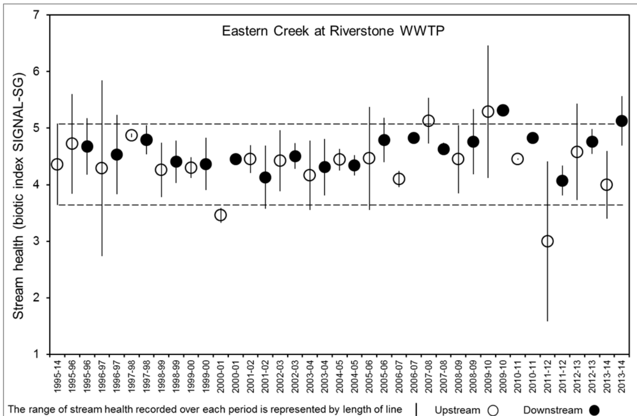
Figure 4-9 Ecological monitoring control chart for Eastern Creek at Riverstone
