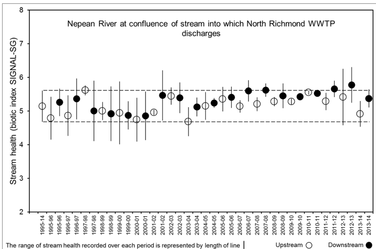
Figure 4-16 Ecological monitoring control chart for Nepean River at North Richmond
