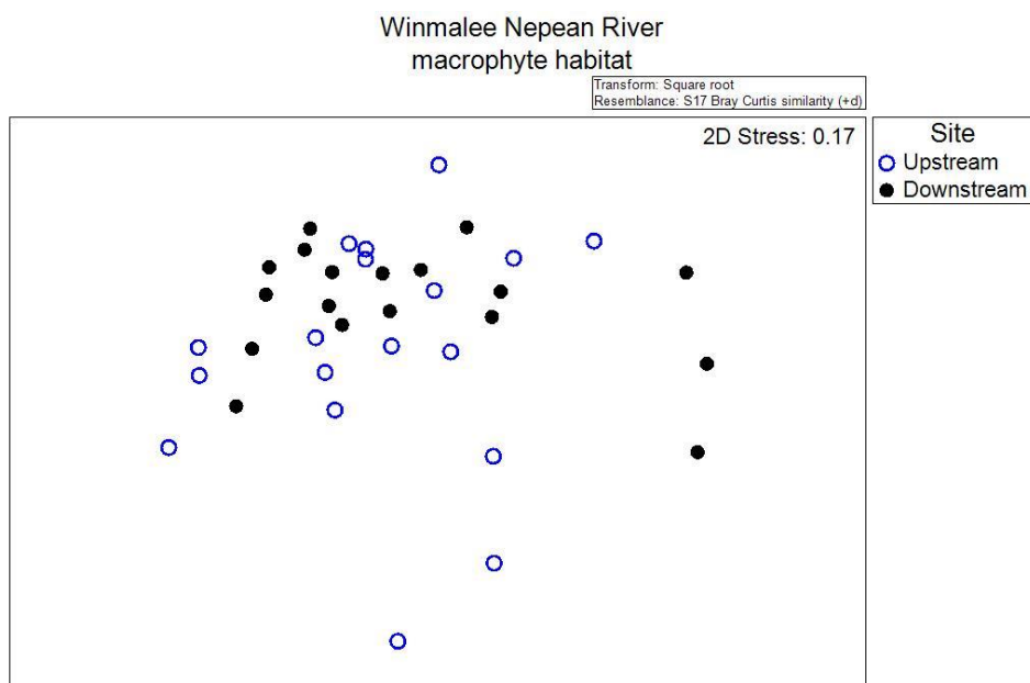
Figure 4-21 Two-dimensional ordination plot of freshwater macroinvertebrate macrophyte habitat community structure of Hawkesbury Nepean River upstream and downstream sites of Winmalee plant
