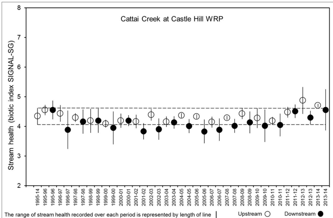
Figure 4-7 Ecological monitoring control chart for Cattai Creek at Castle Hill
