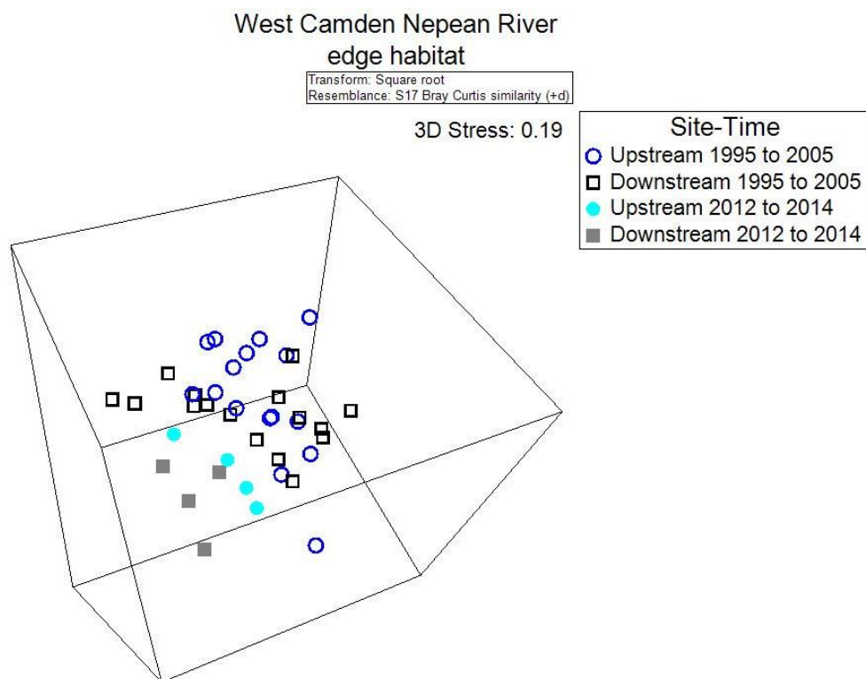
Figure 4-17 Three-dimensional ordination plot of freshwater macroinvertebrate community structure of Hawkesbury Nepean River upstream and downstream sites of West Camden plant for two periods (Period 1 data 1995 to 2005 and Period 2 data from 2012 to 2014)
