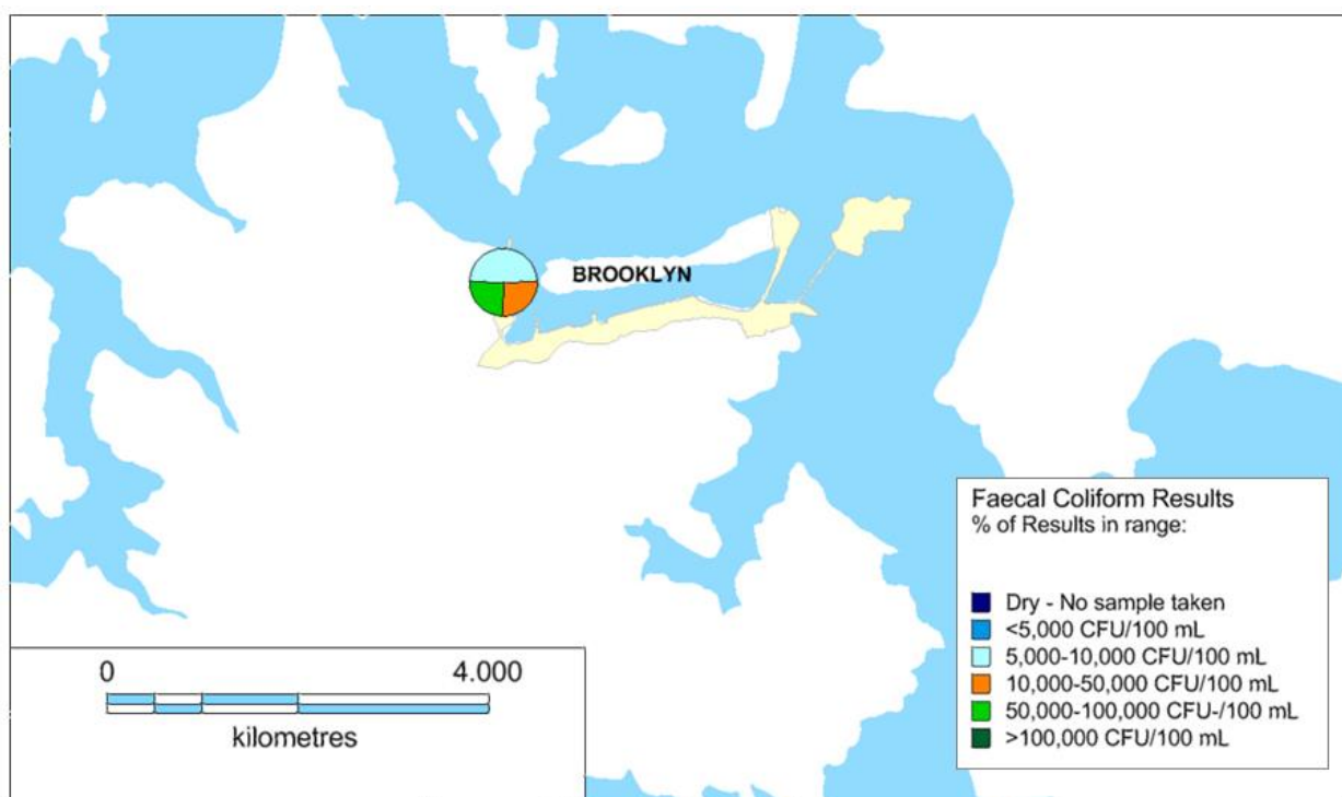
Figure 1-35 Brooklyn SCAMP exceeded the faecal coliform threshold of 5000 cfu/100 mL more than 50% of the time since 2012-13 when monitoring began, with proportion of results exceeding shown
