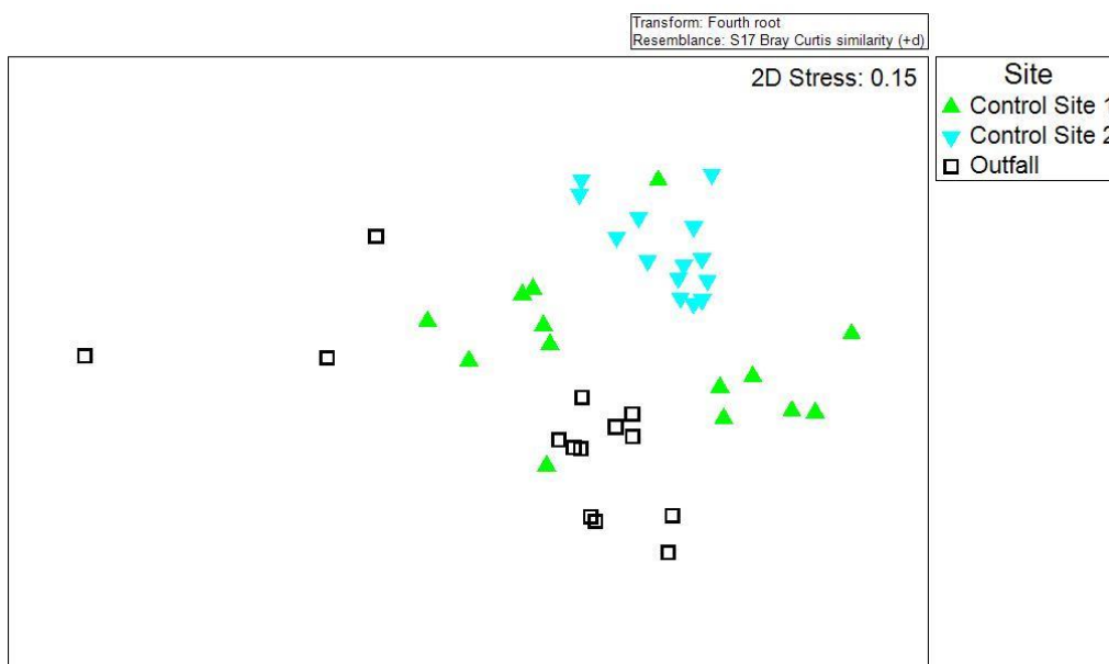
Figure 2-2 Two-dimensional ordination plot of rocky intertidal community structure at Shellharbour outfall and two control sites, with sites colour coded
