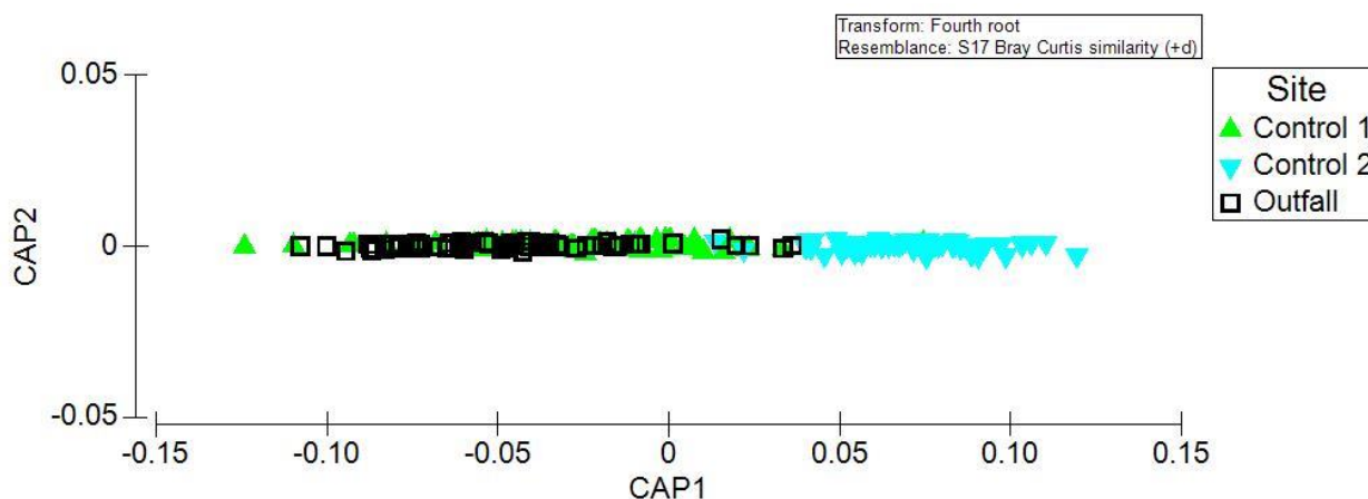
Figure 2-8 CAP ordination plot of rocky intertidal community structure at Shellharbour outfall and two control sites for years 2008 to 2011 and 2013, with site colour coded
