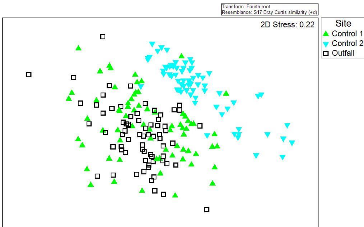
Figure 2-3 Two-dimensional ordination plot of rocky intertidal community structure at Shellharbour outfall and two control sites for years 2008 to 2011 and 2013, with sites colour coded
