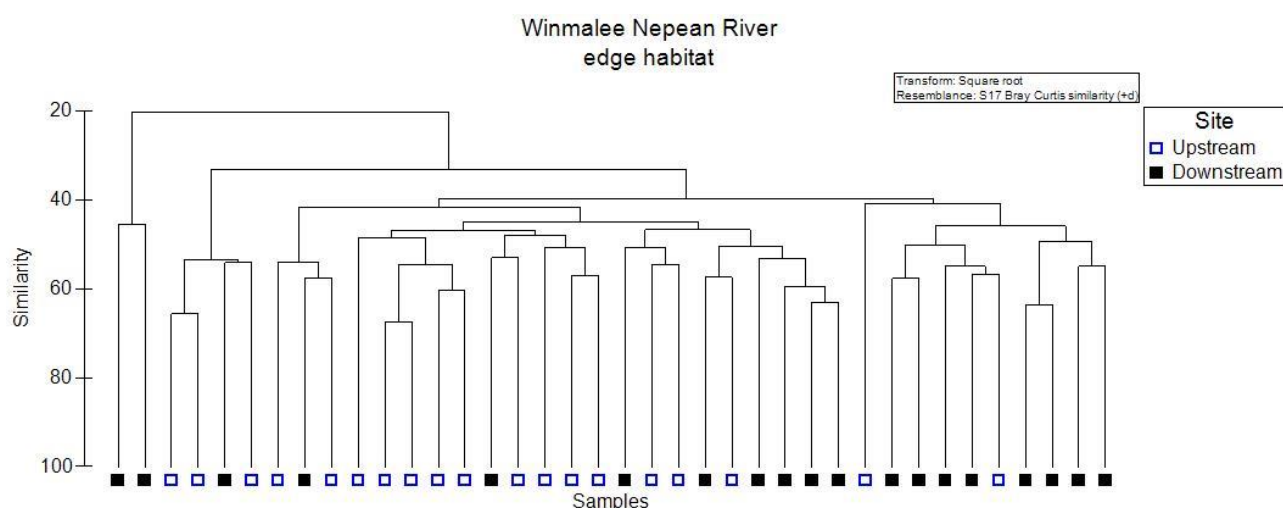
Figure 4-25 Tree diagram of freshwater macroinvertebrate edge habitat community structure of Hawkesbury Nepean River upstream and downstream sites of Winmalee plant
