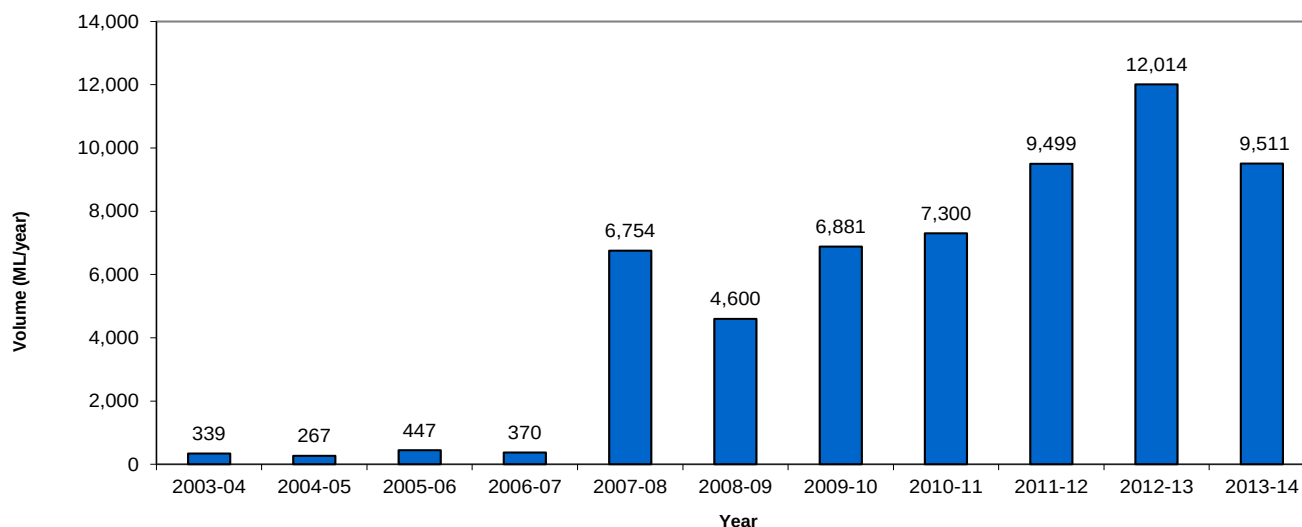
Figure 1-36 Previous ten years of recycled water volumes from all ocean plants
