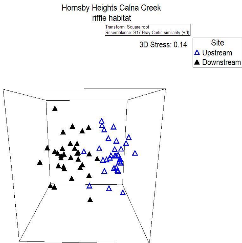
Figure 4-32 Three-dimensional ordination plot of freshwater macroinvertebrate riffle habitat community structure of Calna Creek upstream and downstream sites of Hornsby Heights plant
