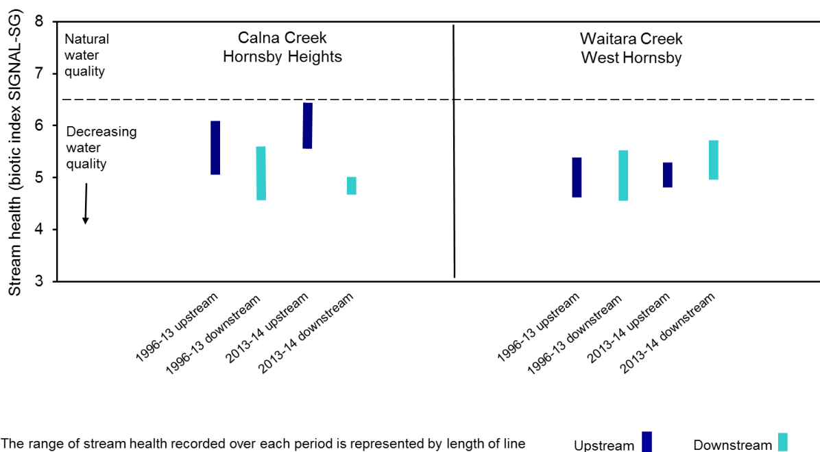
Figure 1-24 Stream health in the Berowra Creek catchment
