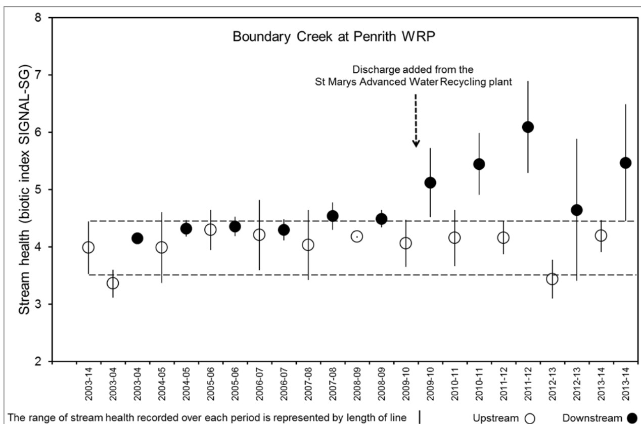
Figure 4-13 Ecological monitoring control chart for Boundary Creek at Penrith
