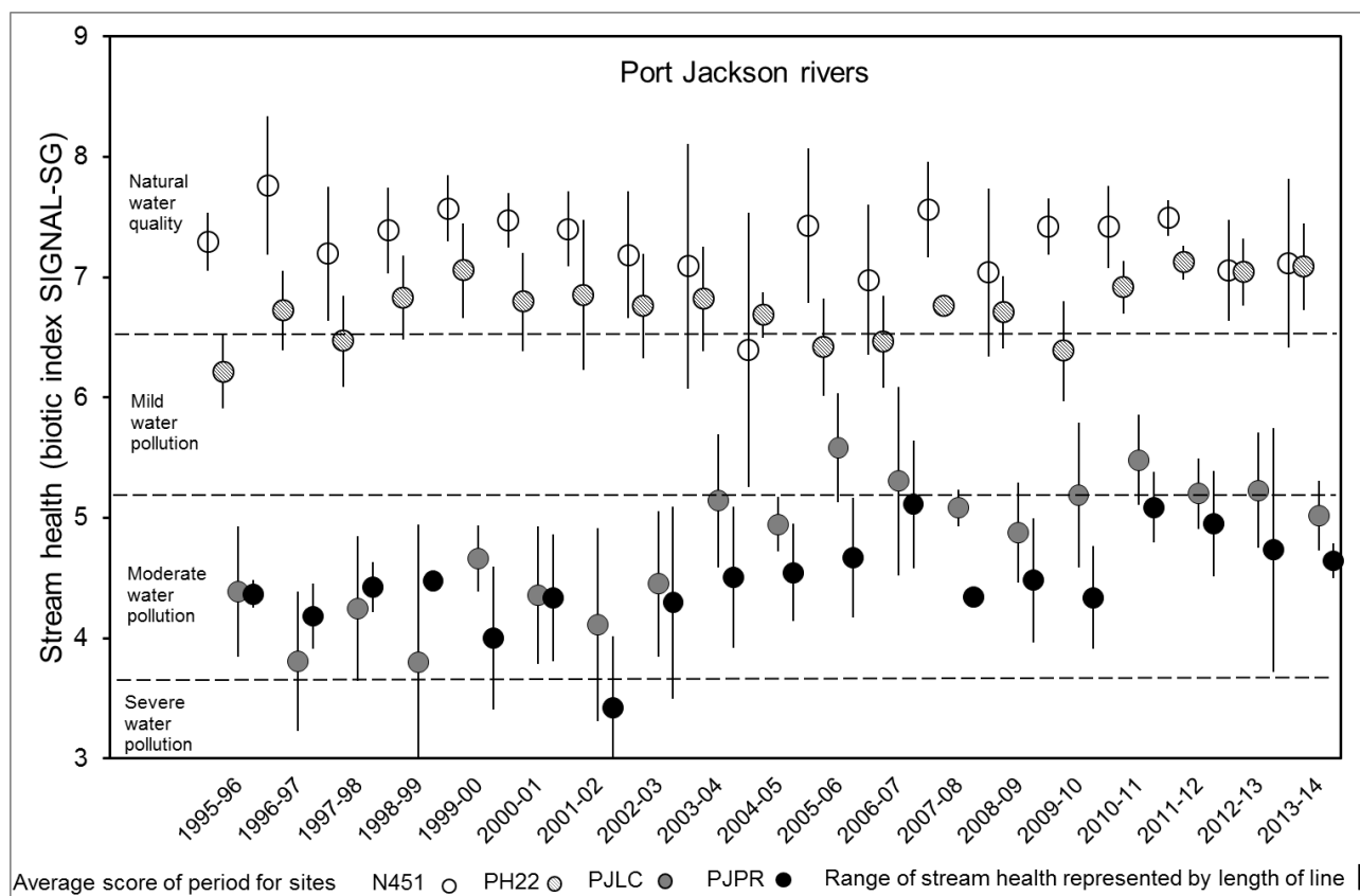
Figure 1-16 Stream health of Lane Cove (PJLC) and Parramatta (PJPR) rivers in comparison to reference site (N451, Lynch's Creek, tributary of Hawkesbury Nepean River; PH22 at McKell Avenue, Hacking River)
