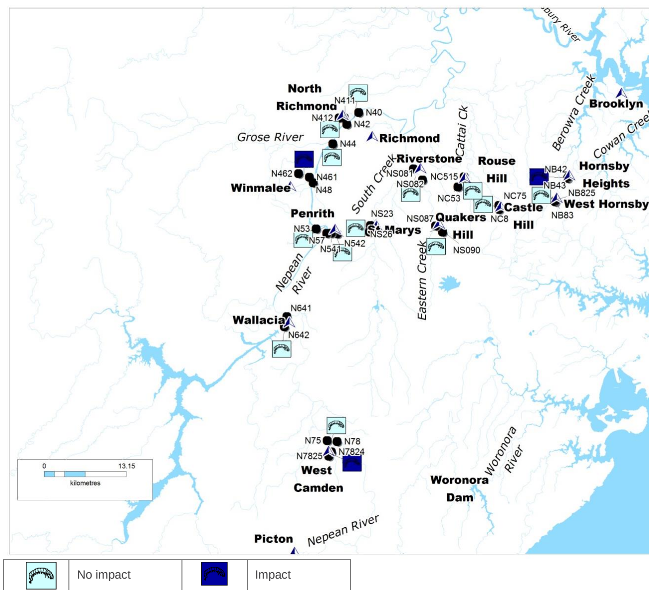
Figure 1-25 Water quality indicator ratings: stream health status at Hawkesbury Nepean River monitoring sites based on macroinvertebrate indicator
