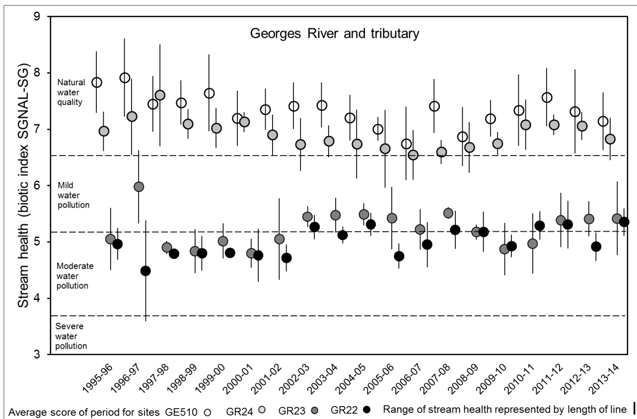
Figure 1-17 Stream health of Georges River sites Liverpool (GR22), Cambridge Causeway (GR23), Ingleburn Reserve (GR24) and O'Hares Creek tributary (GE510)
