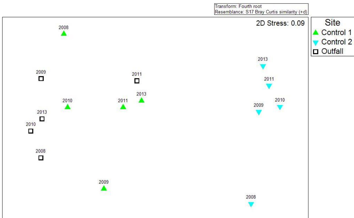
Figure 2-5 Two-dimensional ordination plot of site-year centroids of rocky intertidal community structure at Shellharbour outfall and two control sites for years 2008 to 2011 and 2013
