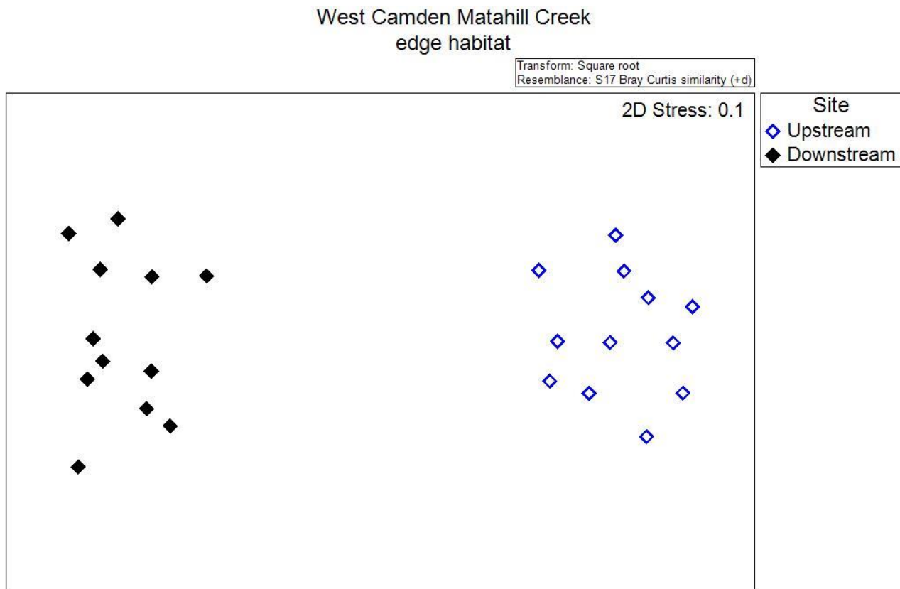
Figure 4-19 Two-dimensional ordination plot of freshwater macroinvertebrate community structure of Matahill Creek upstream and downstream sites of West Camden plant
