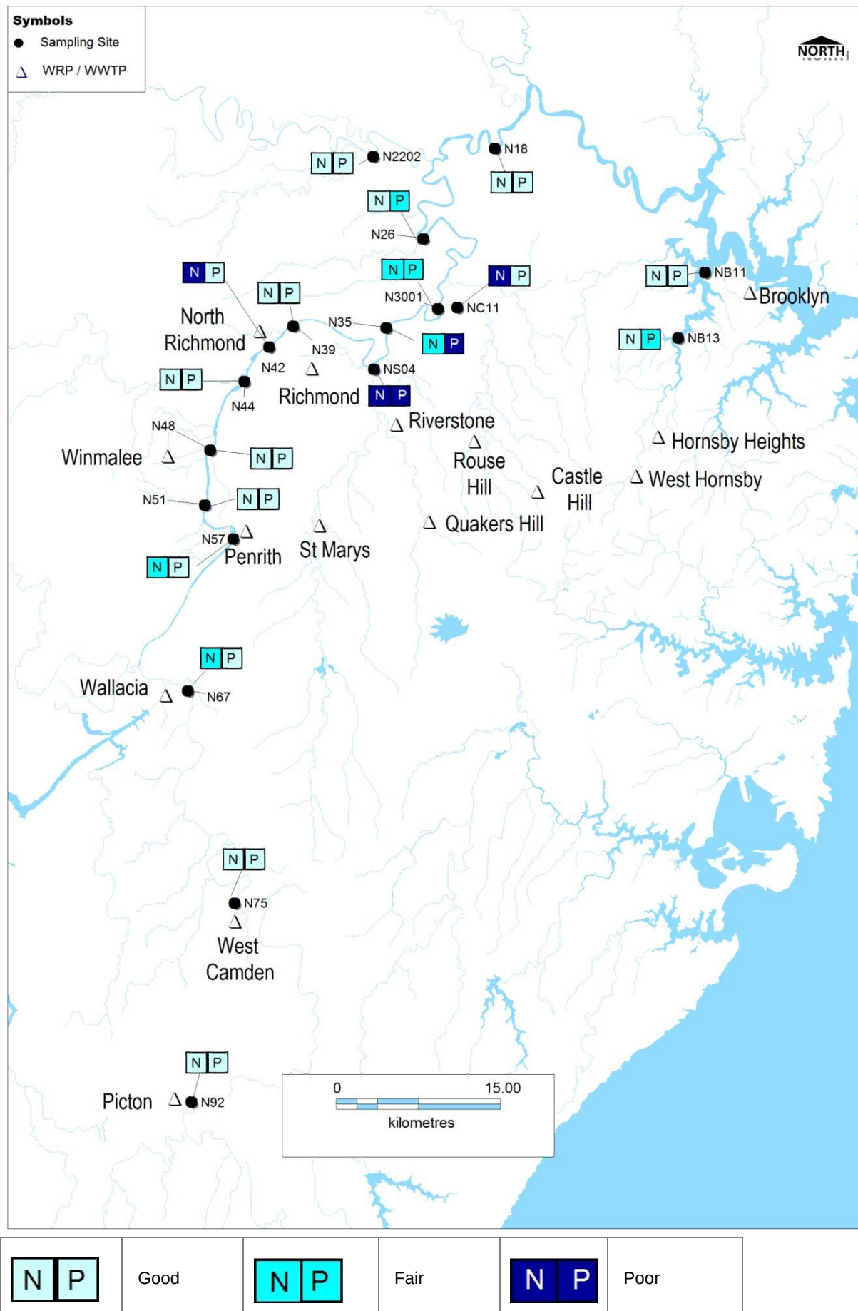
Figure 1-26 Water quality ratings based on total nitrogen and total phosphorus at Hawkesbury Nepean River monitoring sites (2013-14)
