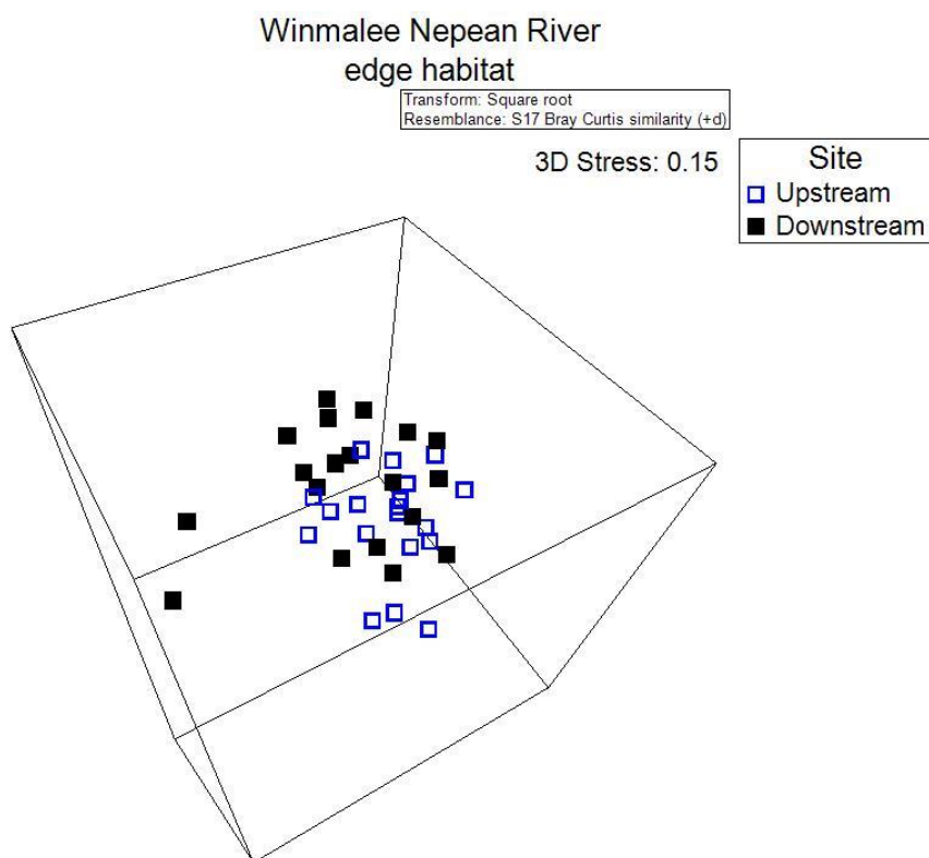
Figure 4-22 Three-dimensional ordination plot of freshwater macroinvertebrate edge habitat community structure of Hawkesbury Nepean River upstream and downstream sites of Winmalee plant
