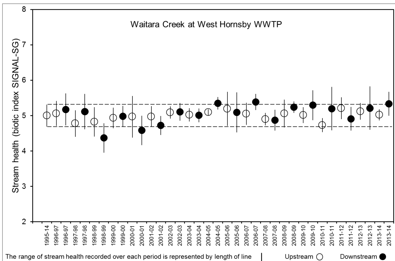
Figure 4-6 Ecological monitoring control chart for Waitara Creek at West Hornsby
