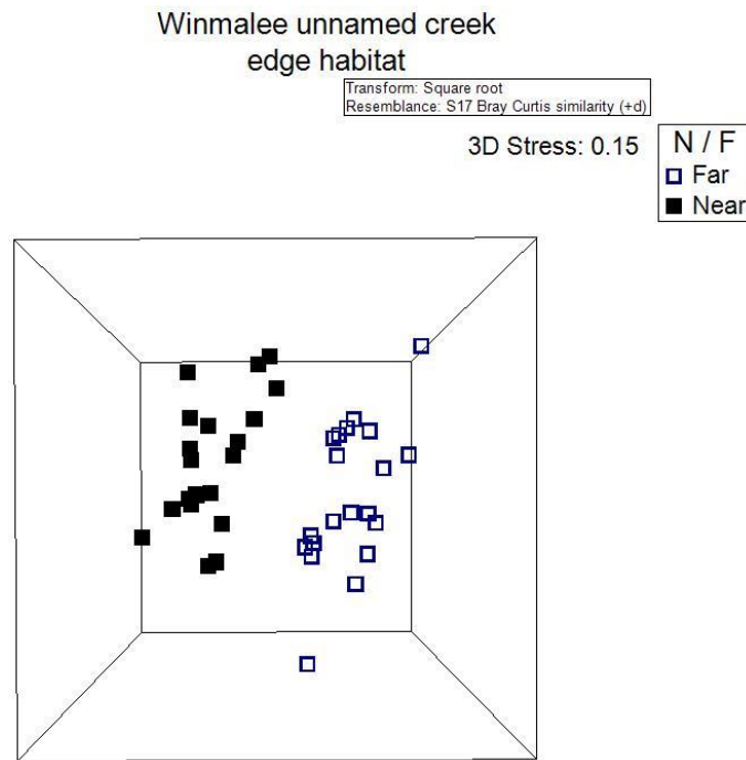
Figure 4-27 Three-dimensional ordination plot of freshwater macroinvertebrate edge habitat community structure of unnamed creek downstream sites of Winmalee plant
