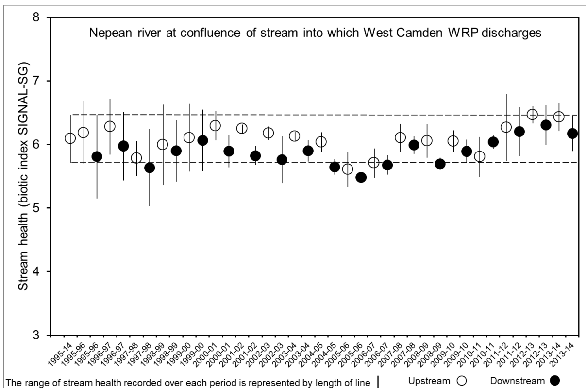
Figure 4-1 Ecological monitoring control chart for Hawkesbury Nepean River at West Camden
