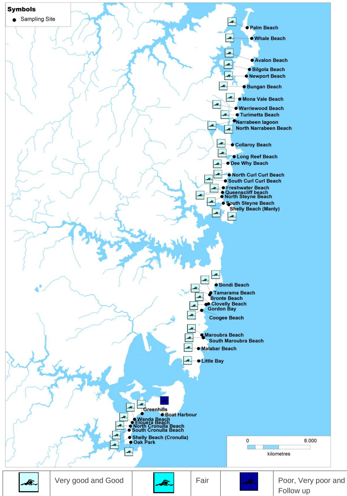
Figure 1-9 Beach Suitability Grades of Sydney beaches 2013-14
