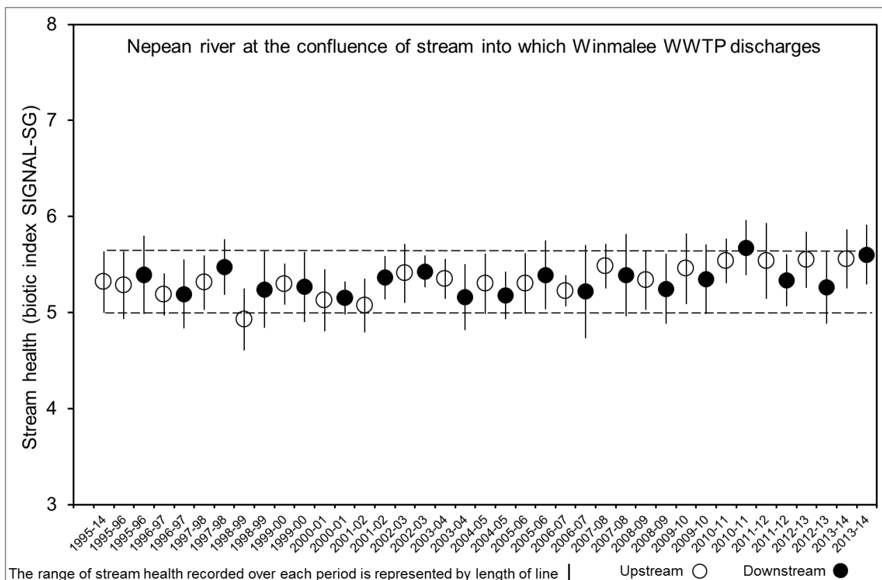
Figure 4-3 Ecological monitoring control chart for Nepean River at Winmalee
