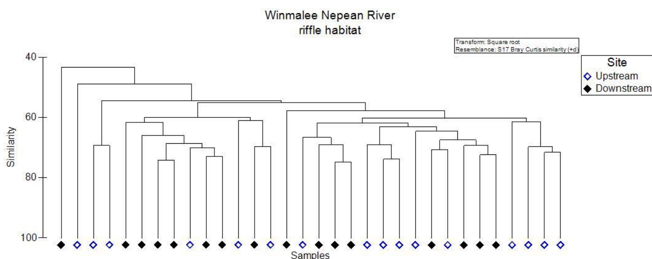
Figure 4-26 Tree diagram of freshwater macroinvertebrate riffle habitat community structure of Hawkesbury Nepean River upstream and downstream sites of Winmalee plant
