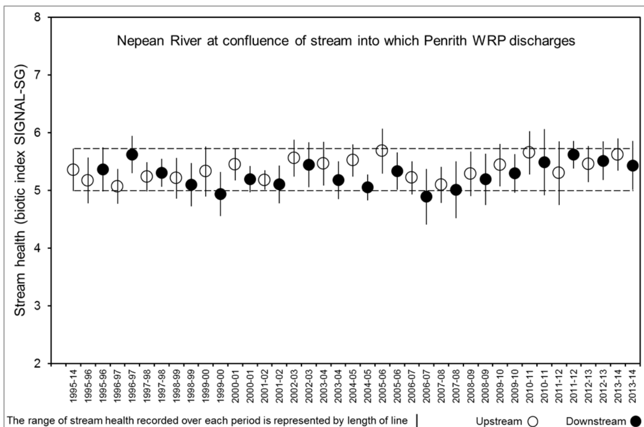
Figure 4-14 Ecological monitoring control chart for Nepean River at Penrith
