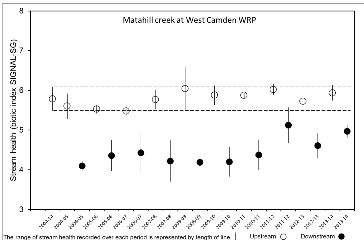
Figure 4-2 Ecological monitoring control chart for Matahill Creek at West Camden
