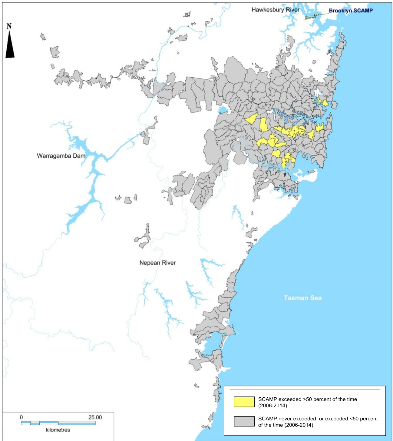
Figure 1-33 SCAMPs that have exceeded the faecal coliform threshold of 5000 cfu/100 mL more than 50% of the time since 2006
