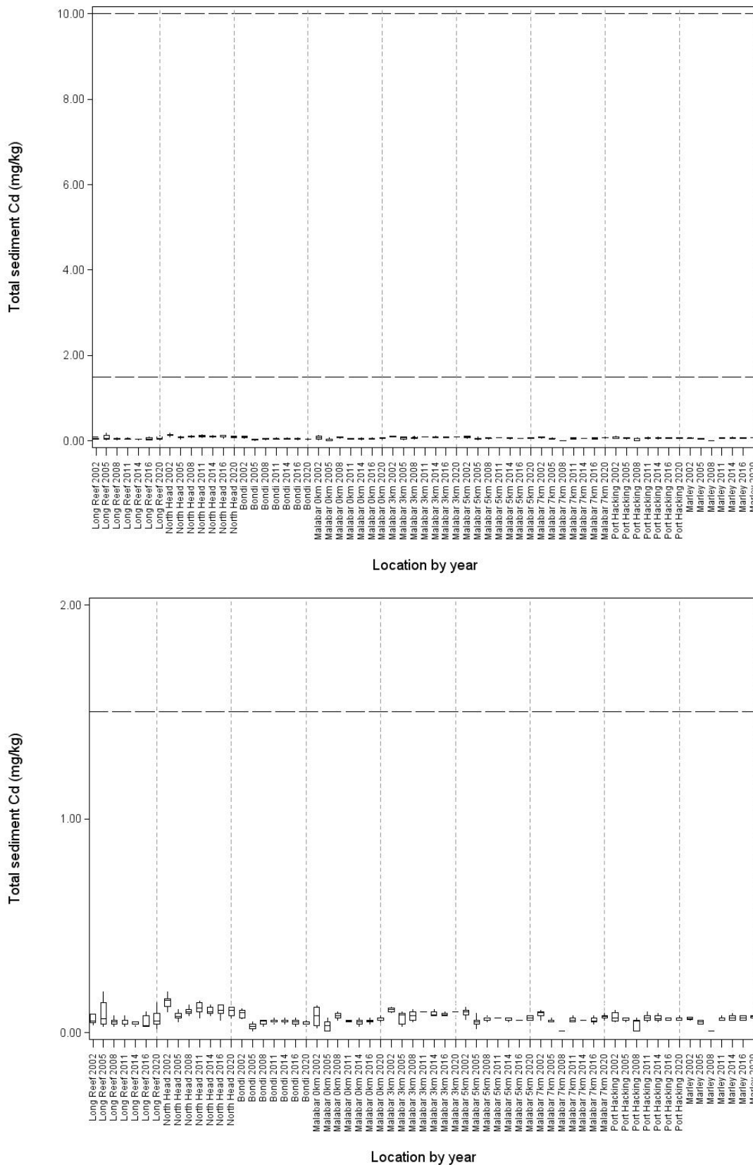
Figure 6-5 Total sedimentary cadmium (Cd) metal concentrations at each location by assessment year Top plot with SQG ERM and ERL values; Bottom plot with SQG ERL value
