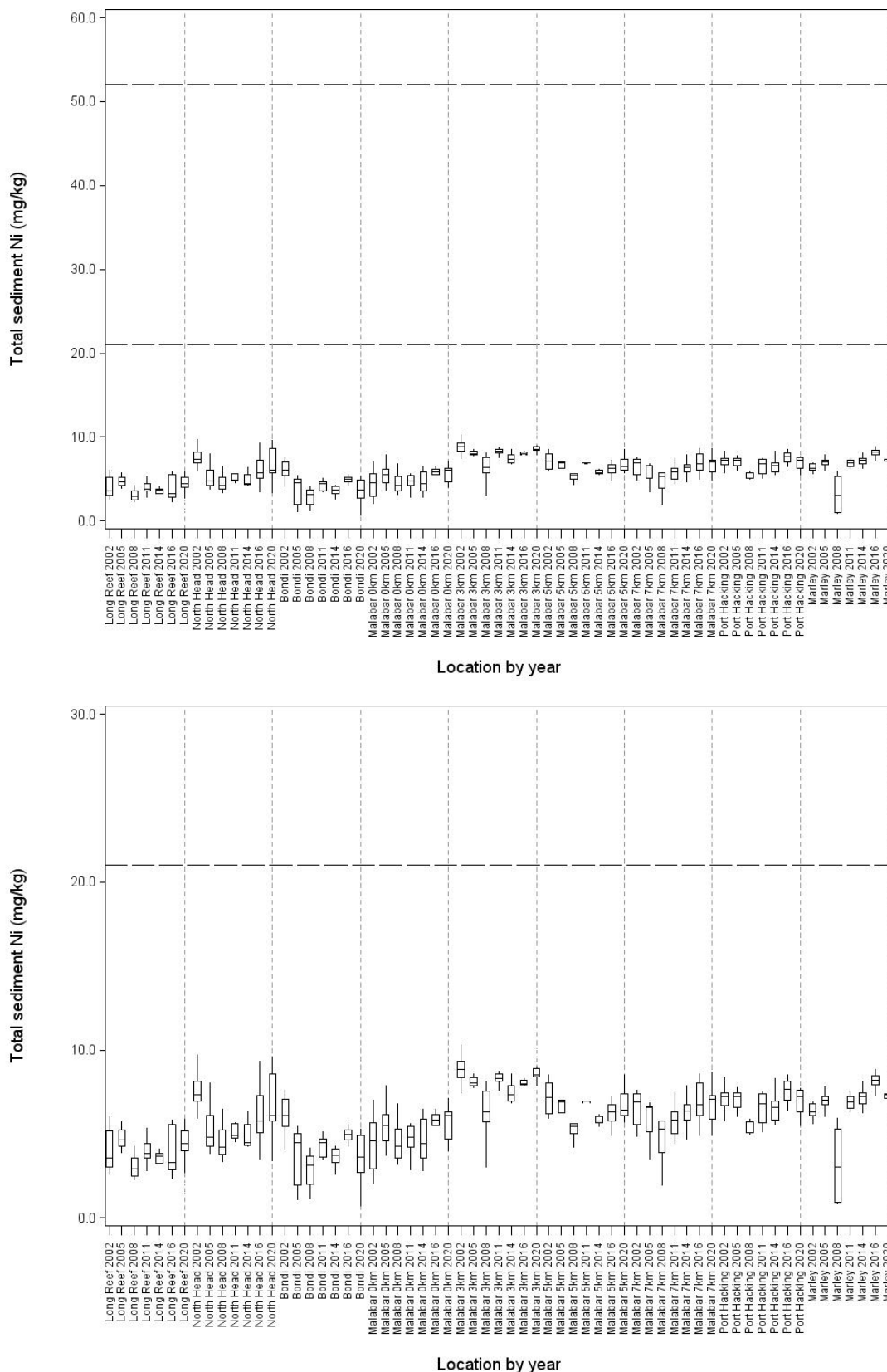
Figure 6-10 Total sedimentary nickel (Ni) metal concentrations at each location by assessment year Top plot with SQG ERM and ERL values; Bottom plot with SQG ERL value
