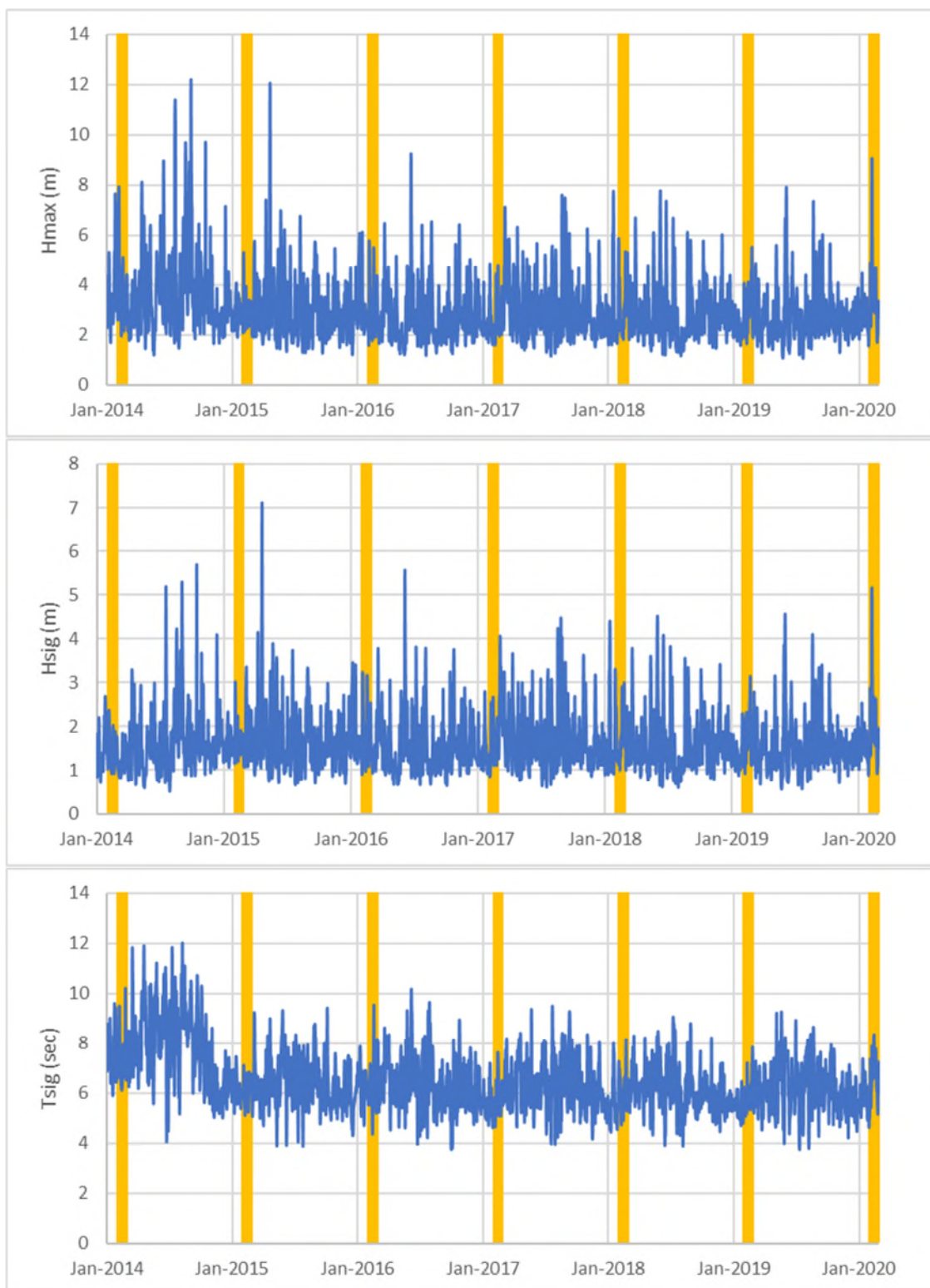
Figure 1 Daily maximum wave height, significant wave height and significant wave period from 1 January 2014 to 29 February 2020. Data obtained from the Ocean Reference Station. Vertical yellow bars indicate February of each year – the month during which sediment sampling was undertaken.
