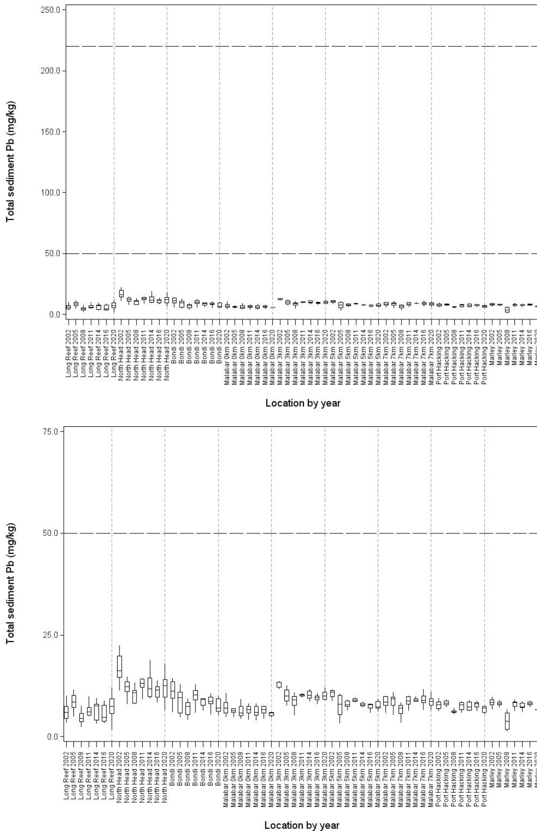
Figure 6-8 Total sedimentary lead (Pb) metal concentrations at each location by assessment year Top plot with SQG ERM and ERL values; Bottom plot with SQG ERL value
