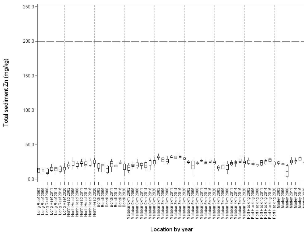
Figure 6-12 Total sedimentary zinc (Zn) metal concentrations at each location by assessment year Top plot with SQG ERM and ERL values; Bottom plot with SQG ERL value.
