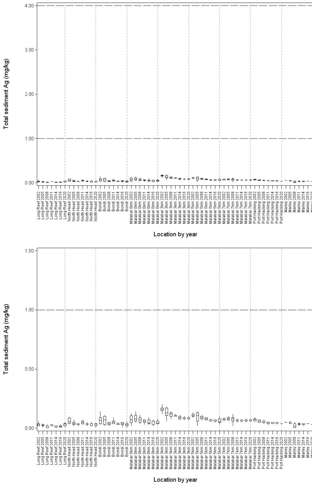
Figure 6-11 Total sedimentary silver (Ag) metal concentrations at each location by assessment year Top plot with SQG ERM and ERL values; Bottom plot with SQG ERL value
