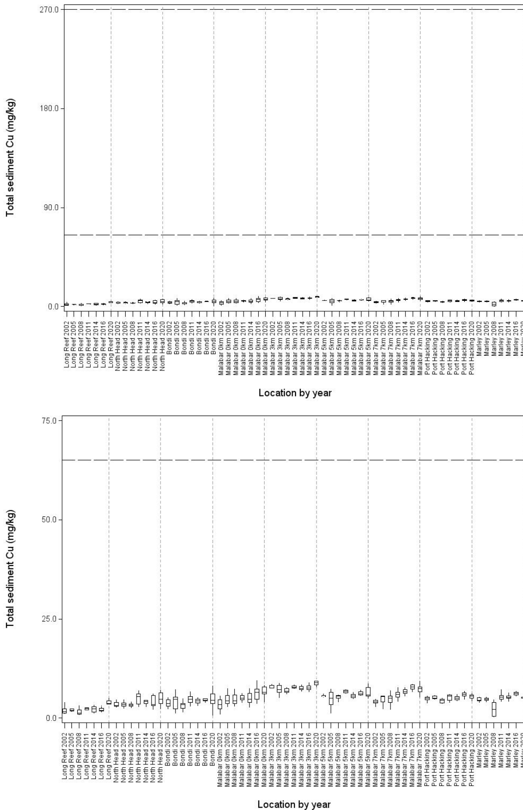
Figure 6-7 Total sedimentary copper (Cu) metal concentrations at each location by assessment year Top plot with SQG ERM and ERL values; Bottom plot with SQG ERL value
