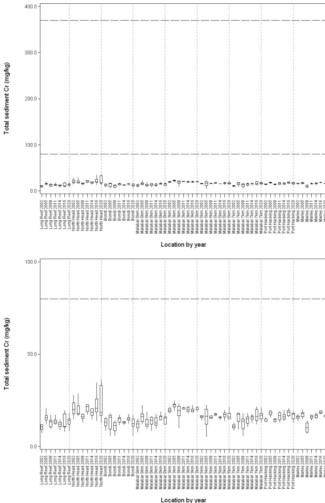
Figure 6-6 Total sedimentary chromium (Cr) metal concentrations at each location by assessment year Top plot with SQG ERM and ERL values; Bottom plot with SQG ERL value
