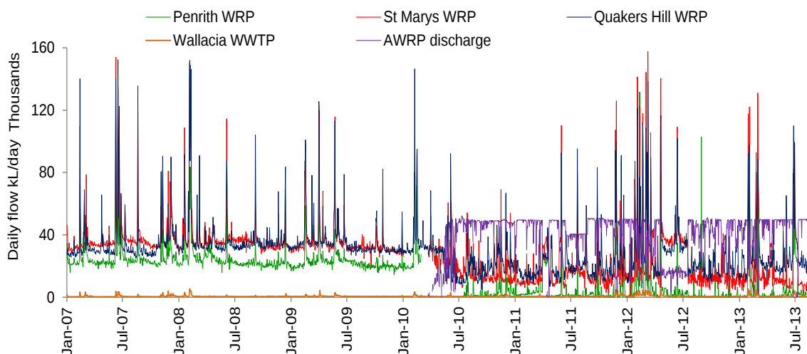
Figure 3-2 Discharges from Penrith, St Marys, Quakers Hill plants and St Marys AWTP
