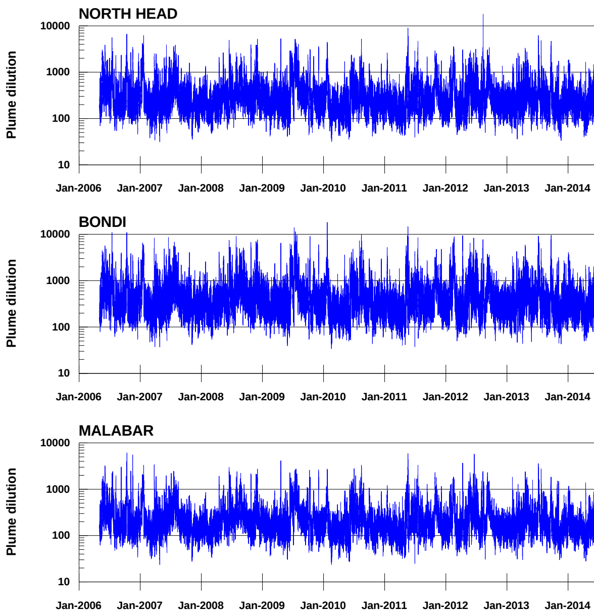
Figure 7-4 Modelled estimates of the plume dilutions for each of the three deepwater ocean outfalls between May 2006 and June 2014
