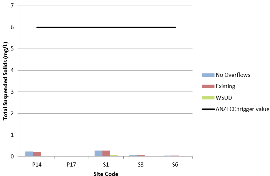
Figure 5-9 Median suspended solids concentrations for sites and scenarios over the ten year period. The ANZECC (2000) aquatic ecosystem default trigger value for lowland coastal rivers in NSW is superimposed
