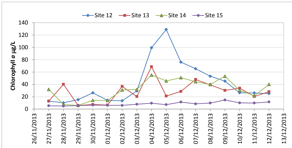
Figure 8-22 Chlorophyll a in the 'event' period for the lake sites and site 15, just downstream of the lake
