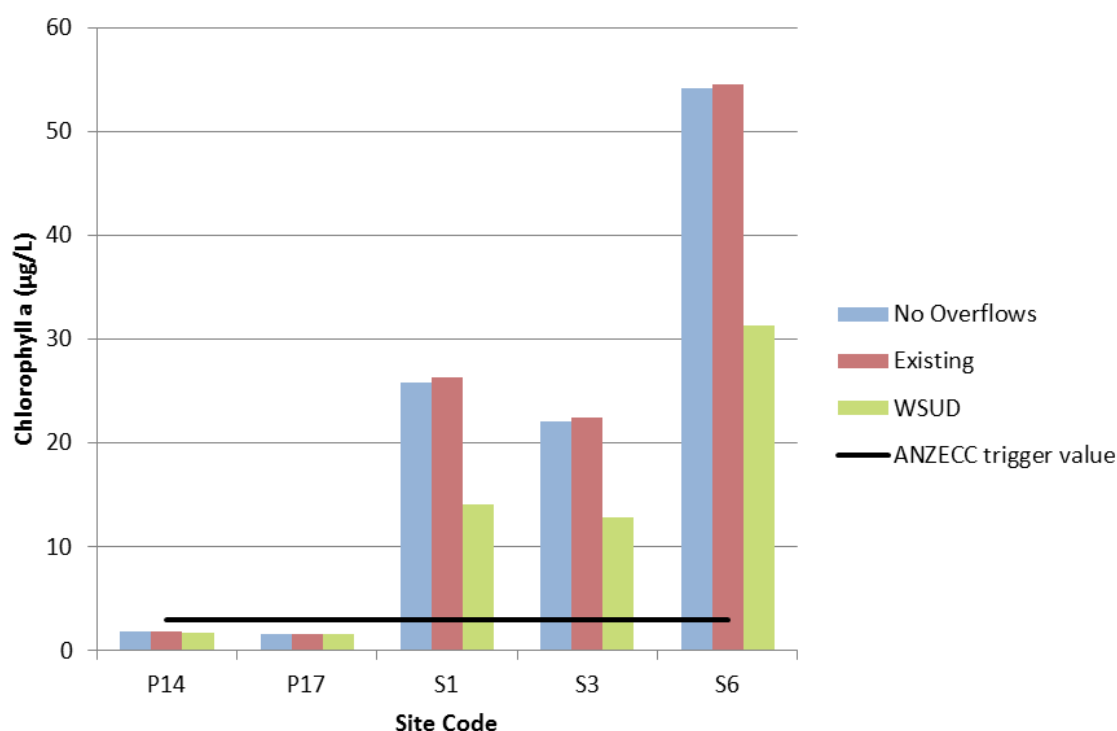
Figure 5-10 Median chlorophyll a concentrations for sites and scenarios over the ten year period. The ANZECC (2000) default trigger value is superimposed
