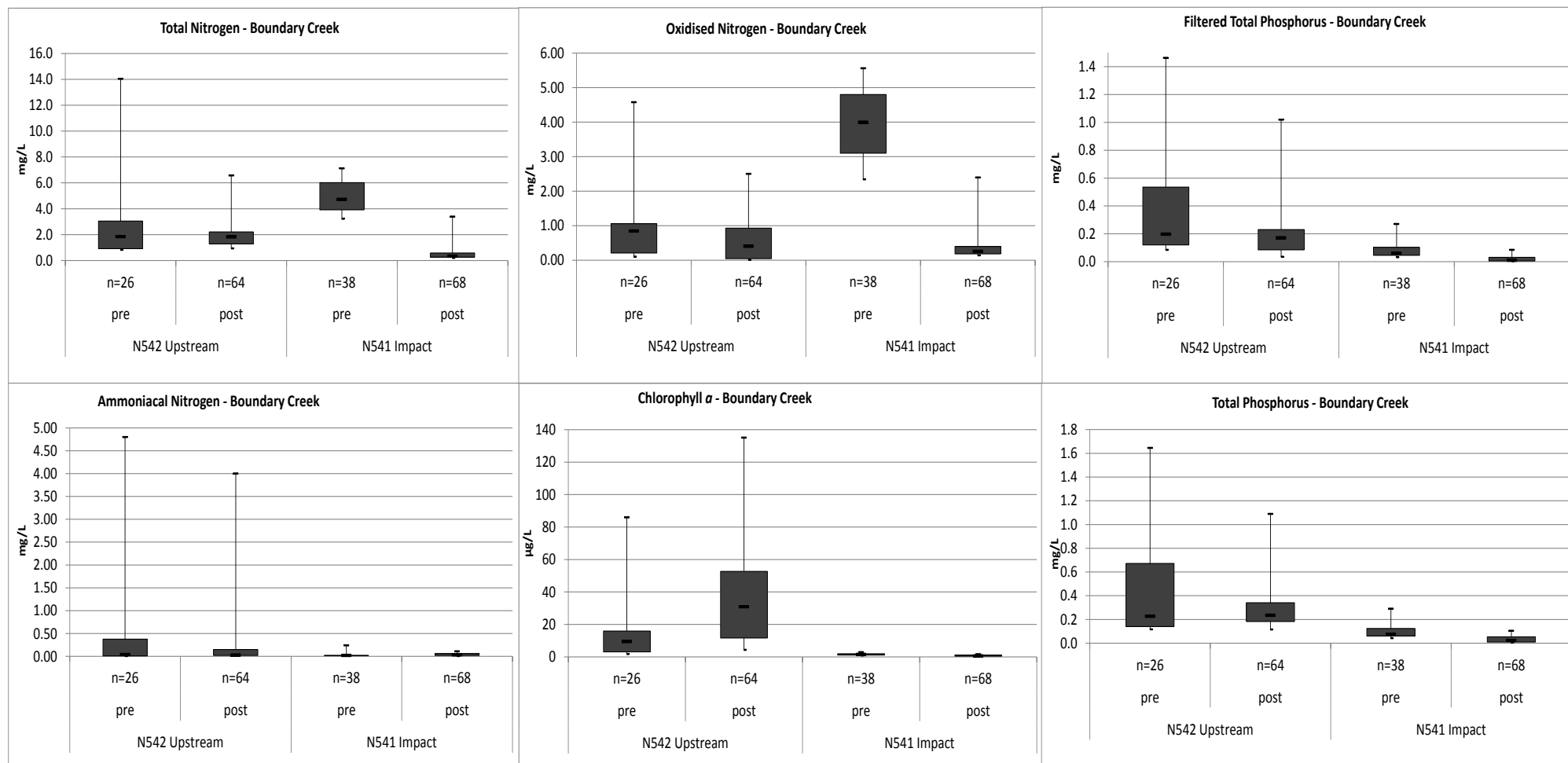
Figure 3-6 Boundary Creek dry weather summary statistics for each site for nutrient parameters and chlorophyll a comparing the pre and post commissioning periods
