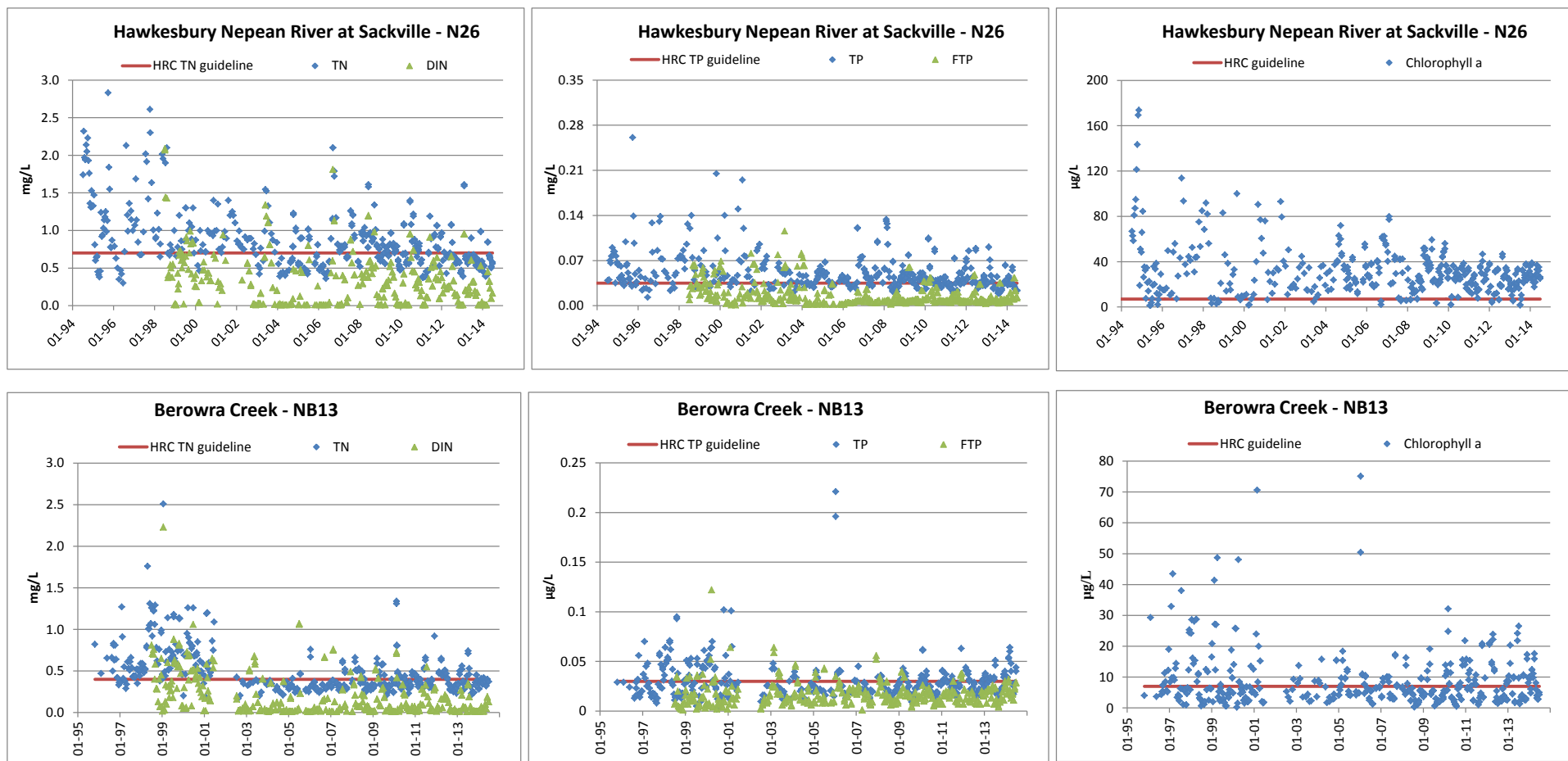
Figure 9-1 Trend analysis temporal plots for Hawkesbury Nepean River sites for total nitrogen (TN) and dissolved inorganic nitrogen (DIN) on the left, total phosphorus (TP) and filtered total phosphorus (FTP) in the middle and chlorophyll a on the right.
