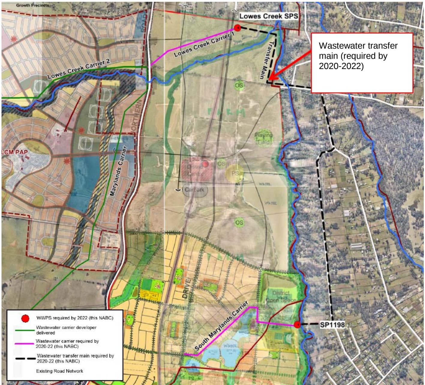
Preferred option – South West Front wastewater
